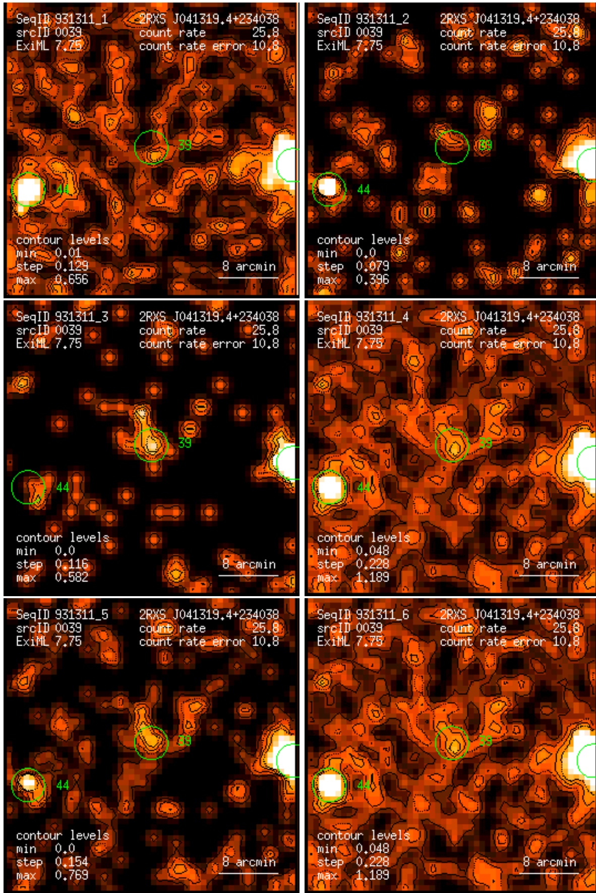
Figure 39: RASS 931311: detection 0039: band rate images, Gaussian filter: (1) PSPC channels 11 – 41, (2) 52 – 90, (3) 91 – 201, (4) 11 – 235, (5) 52 – 201, (6) 11 – 201. Broad band rates in counts/ks. Band rate contour levels in counts/ks/arcmin 2 .
