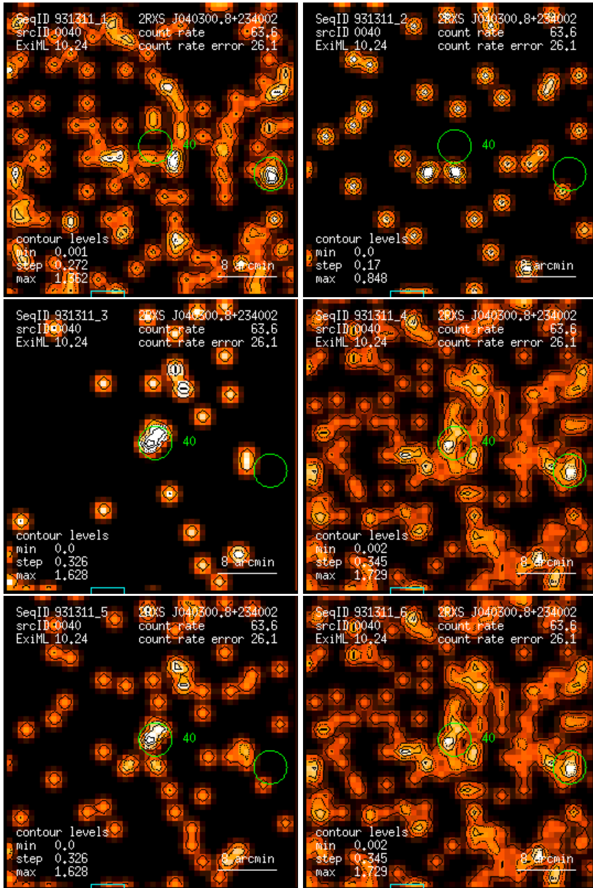
Figure 40: RASS 931311: detection 0040: band rate images, Gaussian filter: (1) PSPC channels 11 – 41, (2) 52 – 90, (3) 91 – 201, (4) 11 – 235, (5) 52 – 201, (6) 11 – 201. Broad band rates in counts/ks. Band rate contour levels in counts/ks/arcmin 2 .
