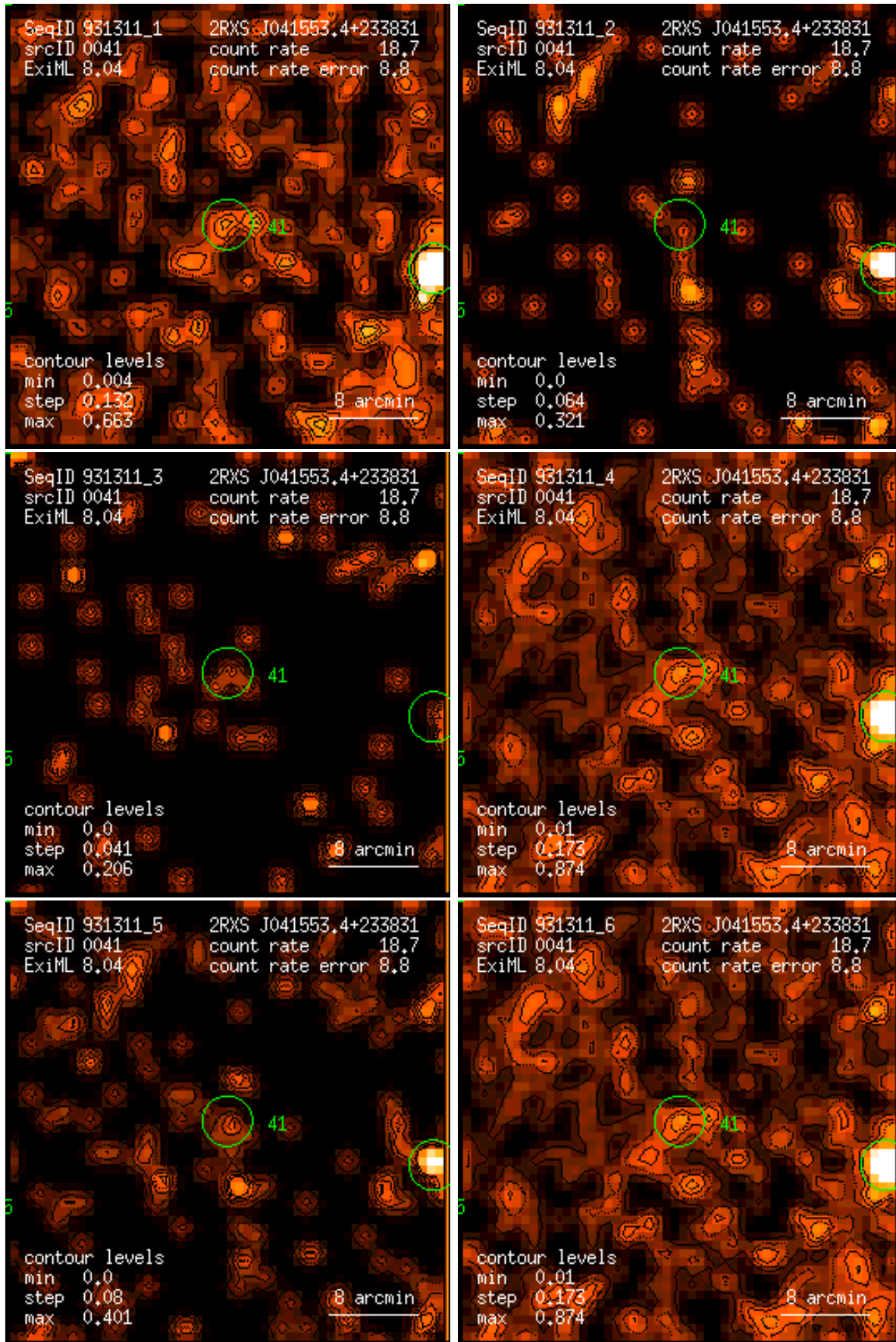
Figure 41: RASS 931311: detection 0041: band rate images, Gaussian filter: (1) PSPC channels 11 – 41, (2) 52 – 90, (3) 91 – 201, (4) 11 – 235, (5) 52 – 201, (6) 11 – 201. Broad band rates in counts/ks. Band rate contour levels in counts/ks/arcmin 2 .
