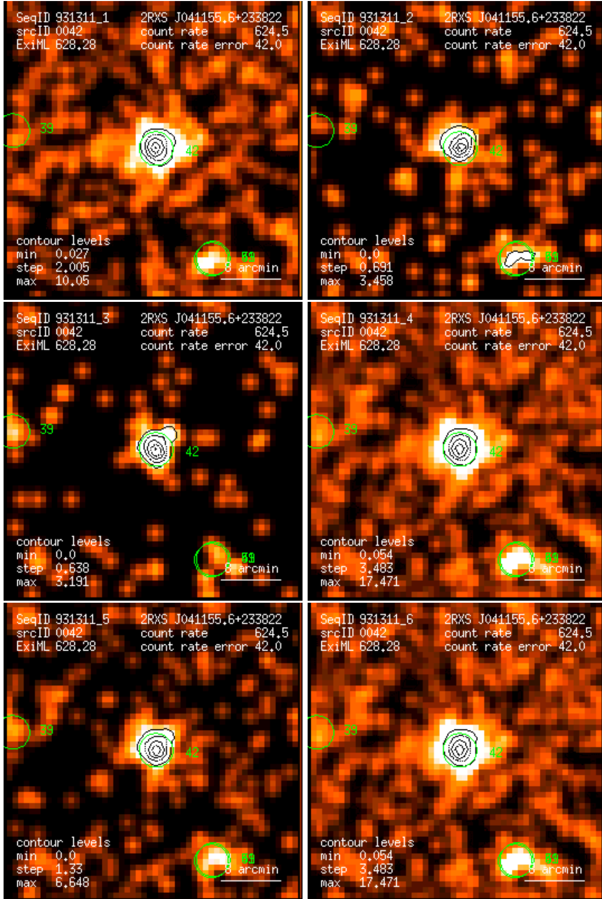
Figure 42: RASS 931311: detection 0042: band rate images, Gaussian filter: (1) PSPC channels 11 – 41, (2) 52 – 90, (3) 91 – 201, (4) 11 – 235, (5) 52 – 201, (6) 11 – 201. Broad band rates in counts/ks. Band rate contour levels in counts/ks/arcmin 2 .
