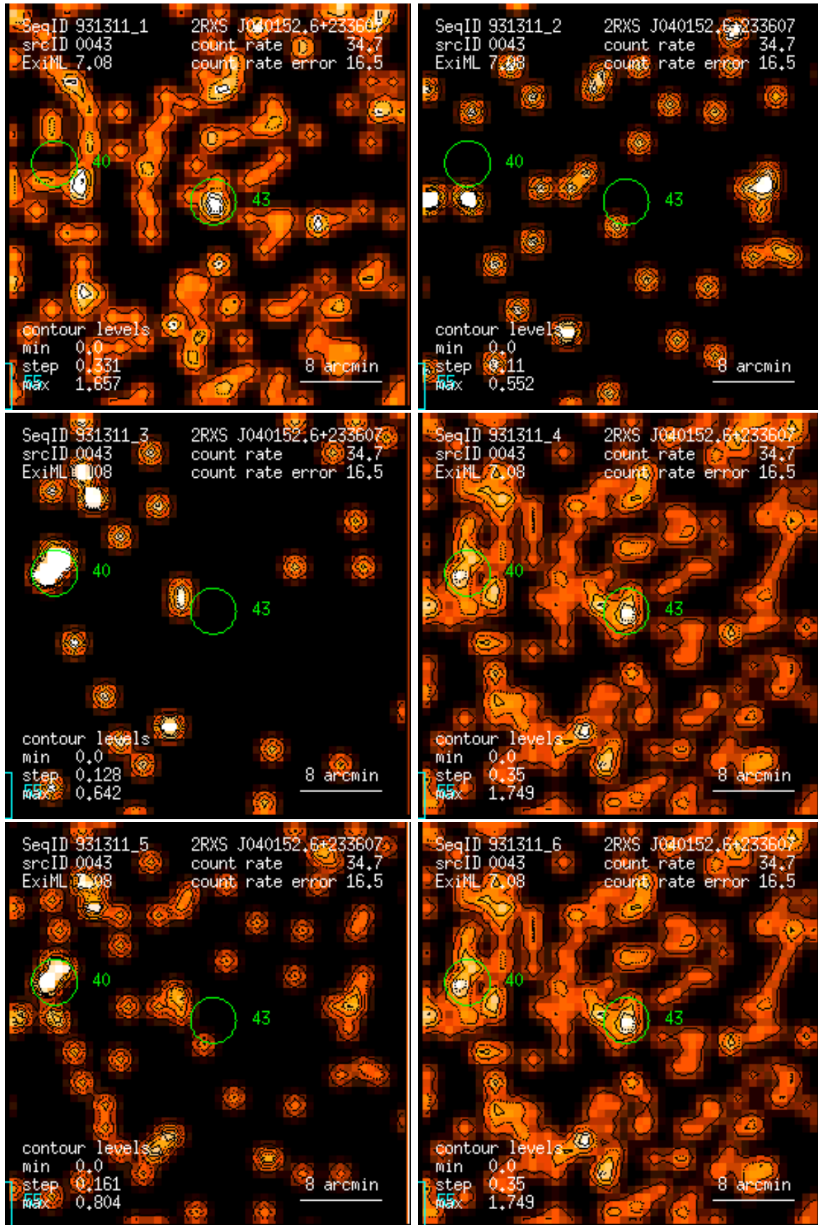
Figure 43: RASS 931311: detection 0043: band rate images, Gaussian filter: (1) PSPC channels 11 – 41, (2) 52 – 90, (3) 91 – 201, (4) 11 – 235, (5) 52 – 201, (6) 11 – 201. Broad band rates in counts/ks. Band rate contour levels in counts/ks/arcmin 2 .
