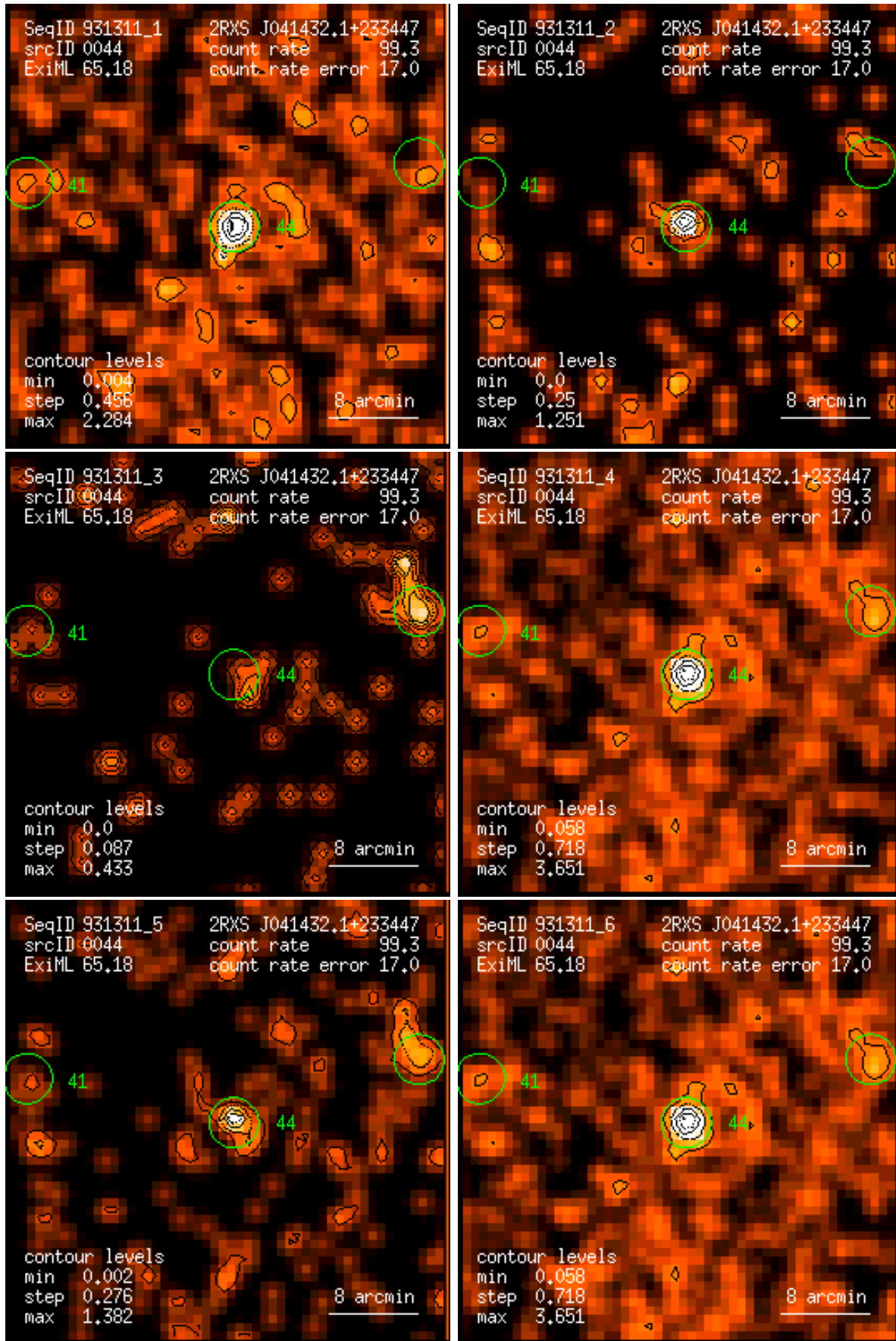
Figure 44: RASS 931311: detection 0044: band rate images, Gaussian filter: (1) PSPC channels 11 – 41, (2) 52 – 90, (3) 91 – 201, (4) 11 – 235, (5) 52 – 201, (6) 11 – 201. Broad band rates in counts/ks. Band rate contour levels in counts/ks/arcmin 2 .
