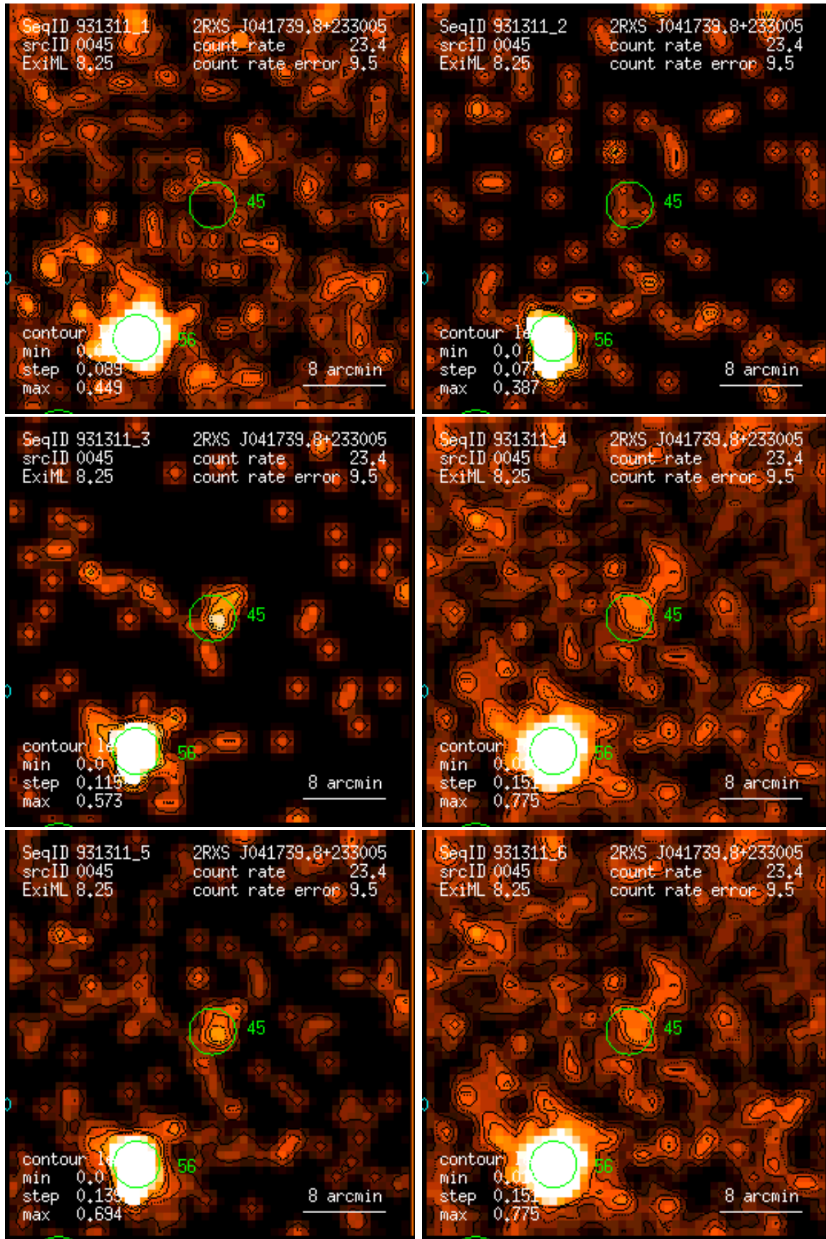
Figure 45: RASS 931311: detection 0045: band rate images, Gaussian filter: (1) PSPC channels 11 – 41, (2) 52 – 90, (3) 91 – 201, (4) 11 – 235, (5) 52 – 201, (6) 11 – 201. Broad band rates in counts/ks. Band rate contour levels in counts/ks/arcmin 2 .
