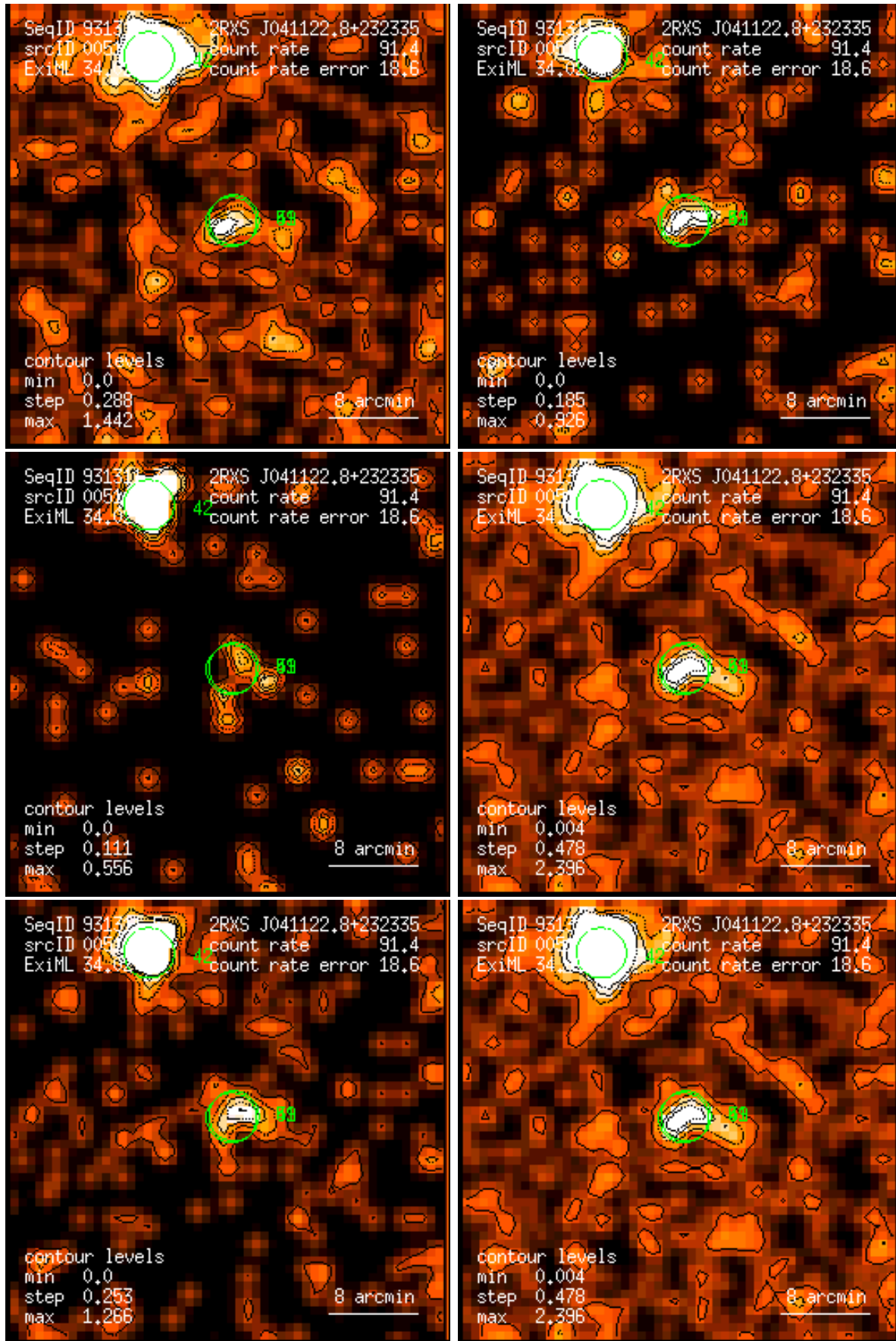
Figure 51: RASS 931311: detection 0051: band rate images, Gaussian filter: (1) PSPC channels 11 – 41, (2) 52 – 90, (3) 91 – 201, (4) 11 – 235, (5) 52 – 201, (6) 11 – 201. Broad band rates in counts/ks. Band rate contour levels in counts/ks/arcmin 2 .
