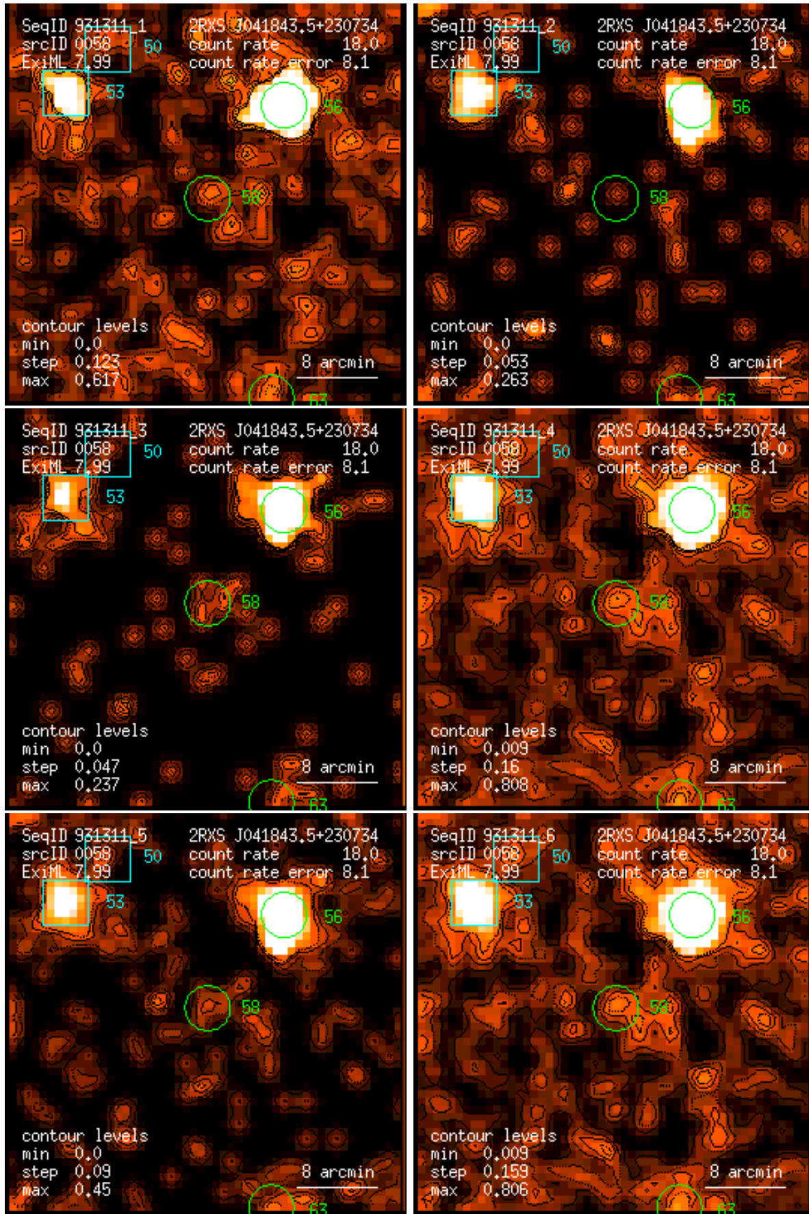
Figure 58: RASS 931311: detection 0058: band rate images, Gaussian filter: (1) PSPC channels 11 – 41, (2) 52 – 90, (3) 91 – 201, (4) 11 – 235, (5) 52 – 201, (6) 11 – 201. Broad band rates in counts/ks. Band rate contour levels in counts/ks/arcmin 2 .
