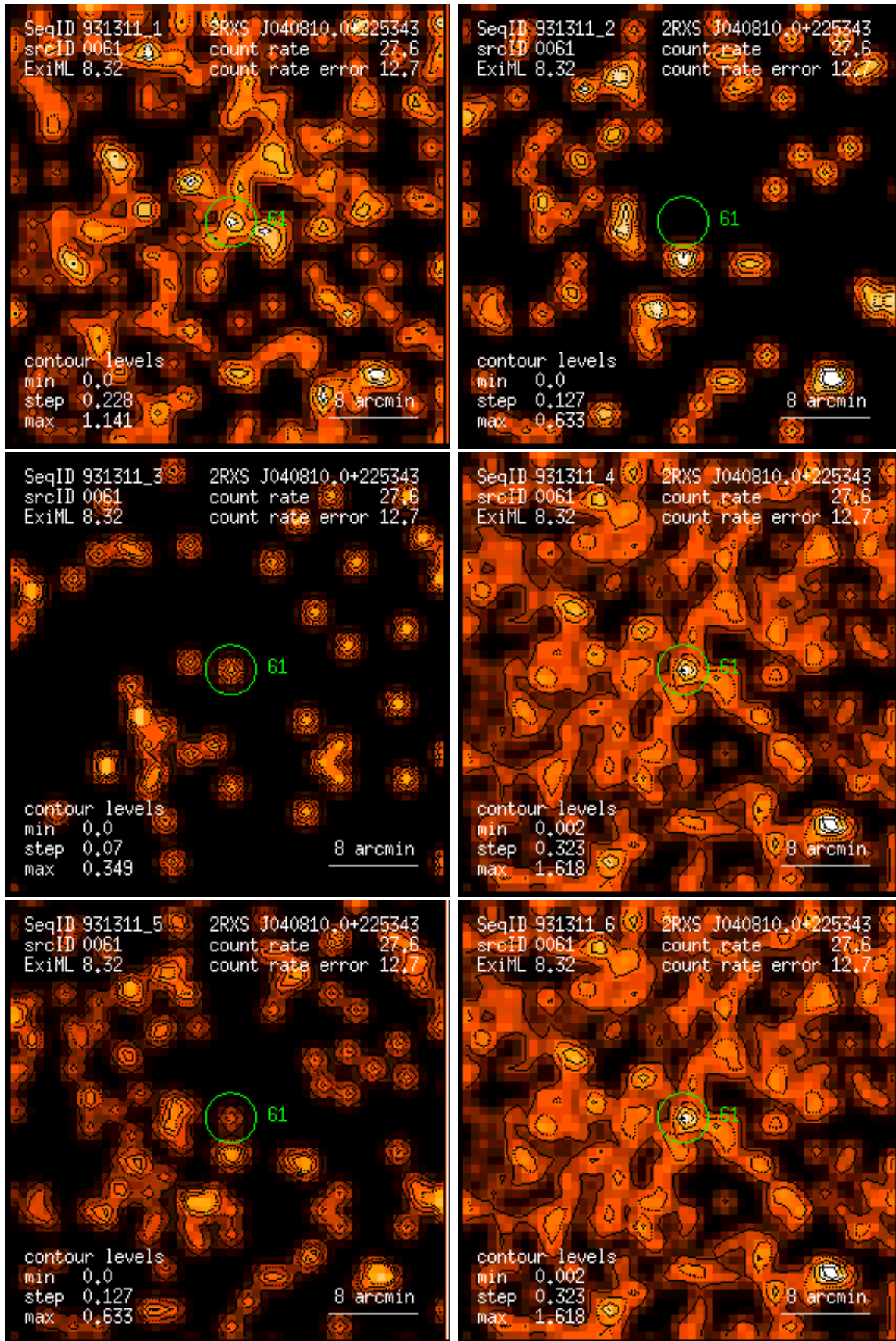
Figure 61: RASS 931311: detection 0061: band rate images, Gaussian filter: (1) PSPC channels 11 – 41, (2) 52 – 90, (3) 91 – 201, (4) 11 – 235, (5) 52 – 201, (6) 11 – 201. Broad band rates in counts/ks. Band rate contour levels in counts/ks/arcmin 2 .
