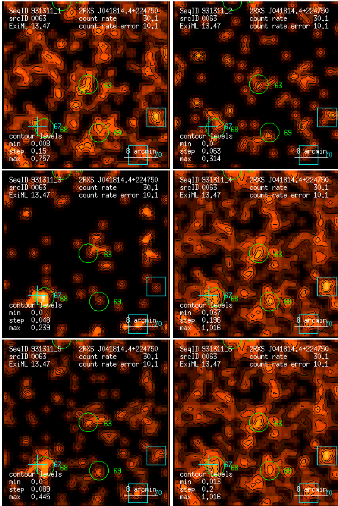
Figure 63: RASS 931311: detection 0063: band rate images, Gaussian filter: (1) PSPC channels 11 – 41, (2) 52 – 90, (3) 91 – 201, (4) 11 – 235, (5) 52 – 201, (6) 11 – 201. Broad band rates in counts/ks. Band rate contour levels in counts/ks/arcmin 2 .
