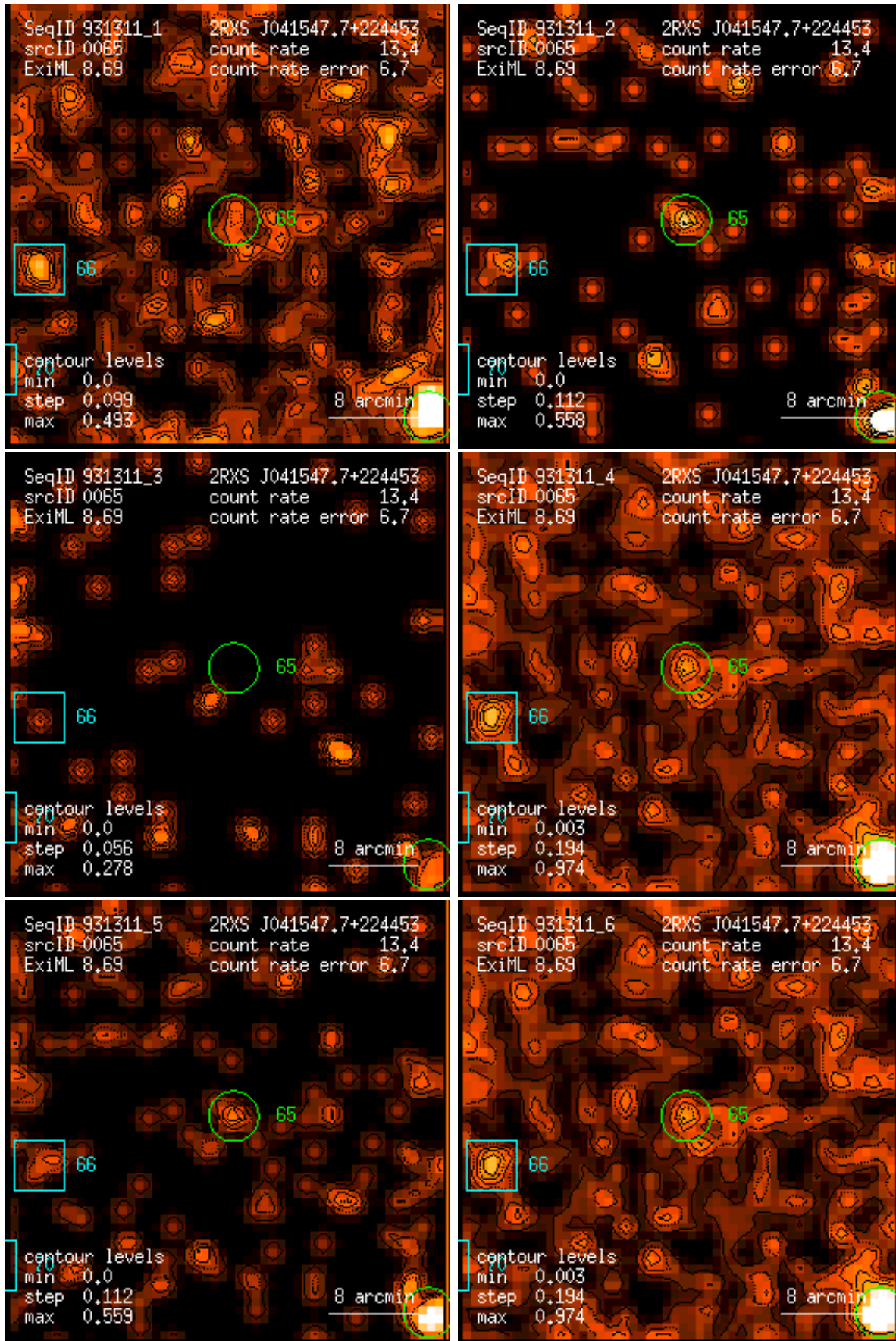
Figure 65: RASS 931311: detection 0065: band rate images, Gaussian filter: (1) PSPC channels 11 – 41, (2) 52 – 90, (3) 91 – 201, (4) 11 – 235, (5) 52 – 201, (6) 11 – 201. Broad band rates in counts/ks. Band rate contour levels in counts/ks/arcmin 2 .
