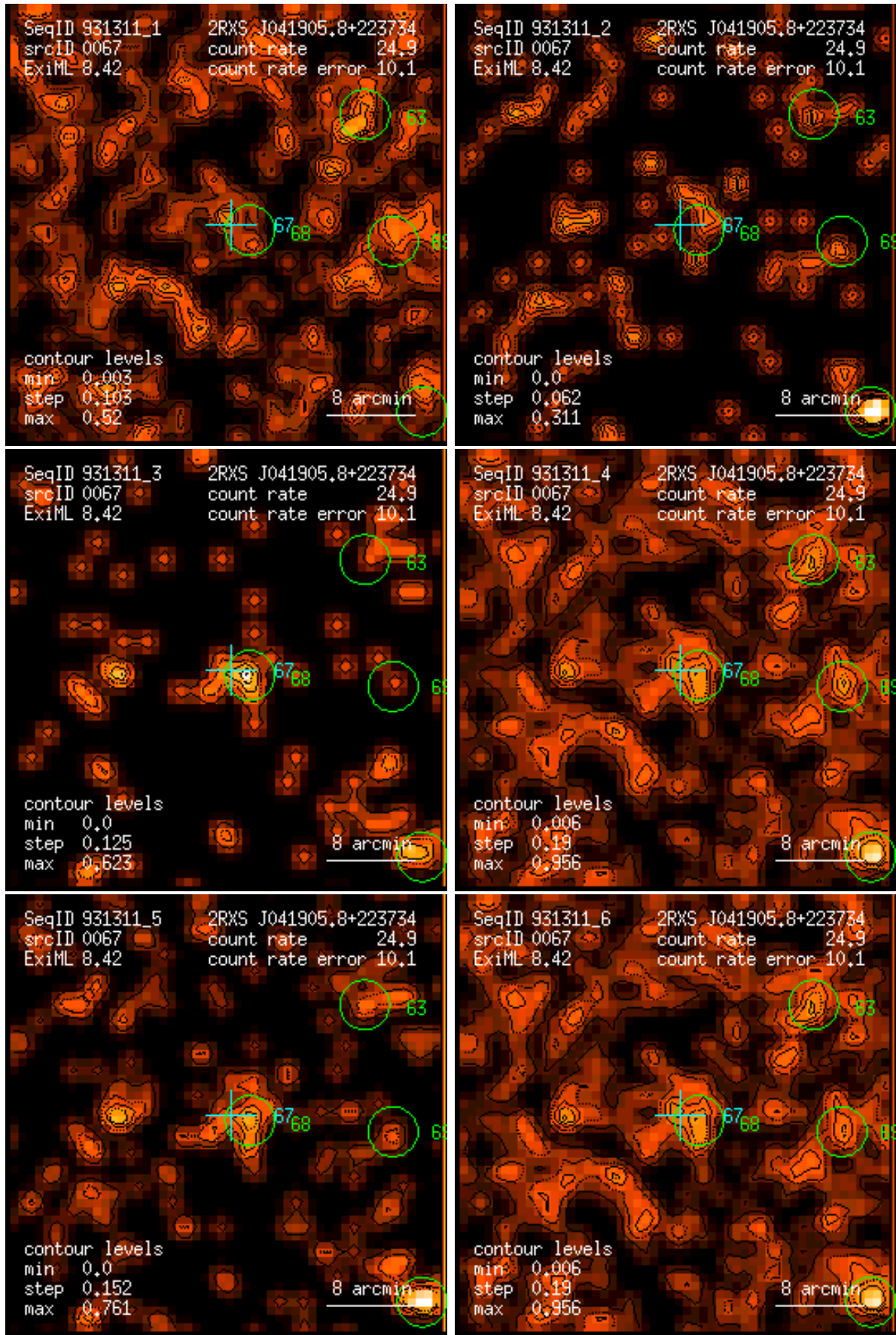
Figure 67: RASS 931311: detection 0067: band rate images, Gaussian filter: (1) PSPC channels 11 – 41, (2) 52 – 90, (3) 91 – 201, (4) 11 – 235, (5) 52 – 201, (6) 11 – 201. Broad band rates in counts/ks. Band rate contour levels in counts/ks/arcmin 2 .
