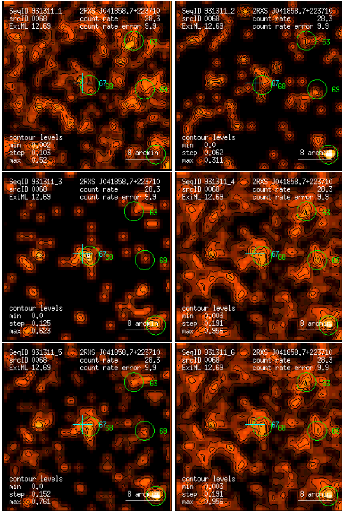
Figure 68: RASS 931311: detection 0068: band rate images, Gaussian filter: (1) PSPC channels 11 – 41, (2) 52 – 90, (3) 91 – 201, (4) 11 – 235, (5) 52 – 201, (6) 11 – 201. Broad band rates in counts/ks. Band rate contour levels in counts/ks/arcmin 2 .
