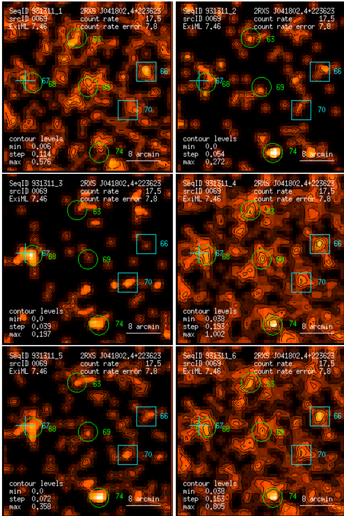
Figure 69: RASS 931311: detection 0069: band rate images, Gaussian filter: (1) PSPC channels 11 – 41, (2) 52 – 90, (3) 91 – 201, (4) 11 – 235, (5) 52 – 201, (6) 11 – 201. Broad band rates in counts/ks. Band rate contour levels in counts/ks/arcmin 2 .
