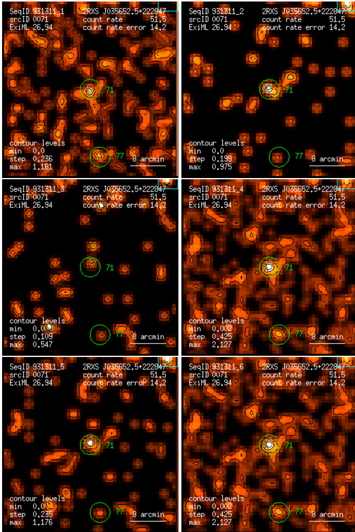
Figure 71: RASS 931311: detection 0071: band rate images, Gaussian filter: (1) PSPC channels 11 – 41, (2) 52 – 90, (3) 91 – 201, (4) 11 – 235, (5) 52 – 201, (6) 11 – 201. Broad band rates in counts/ks. Band rate contour levels in counts/ks/arcmin 2 .
