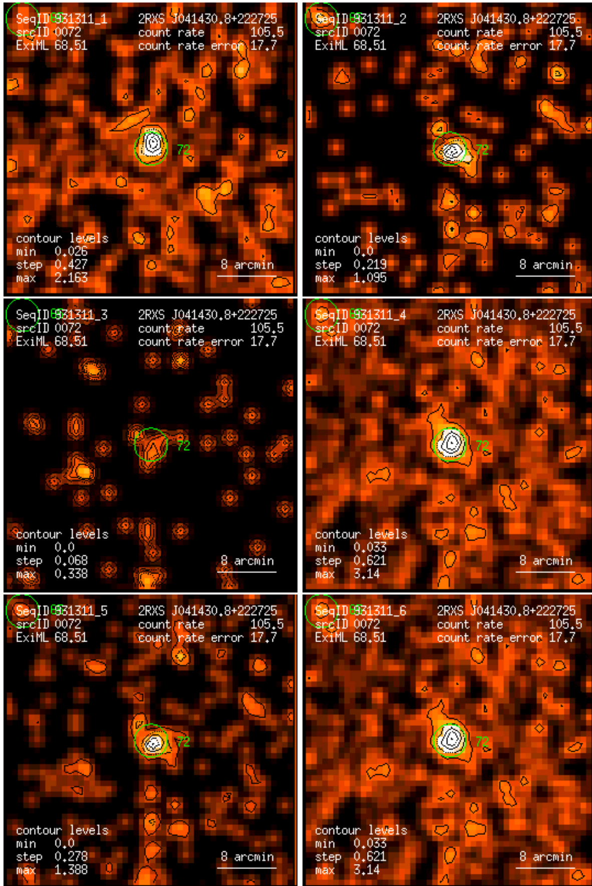
Figure 72: RASS 931311: detection 0072: band rate images, Gaussian filter: (1) PSPC channels 11 – 41, (2) 52 – 90, (3) 91 – 201, (4) 11 – 235, (5) 52 – 201, (6) 11 – 201. Broad band rates in counts/ks. Band rate contour levels in counts/ks/arcmin 2 .
