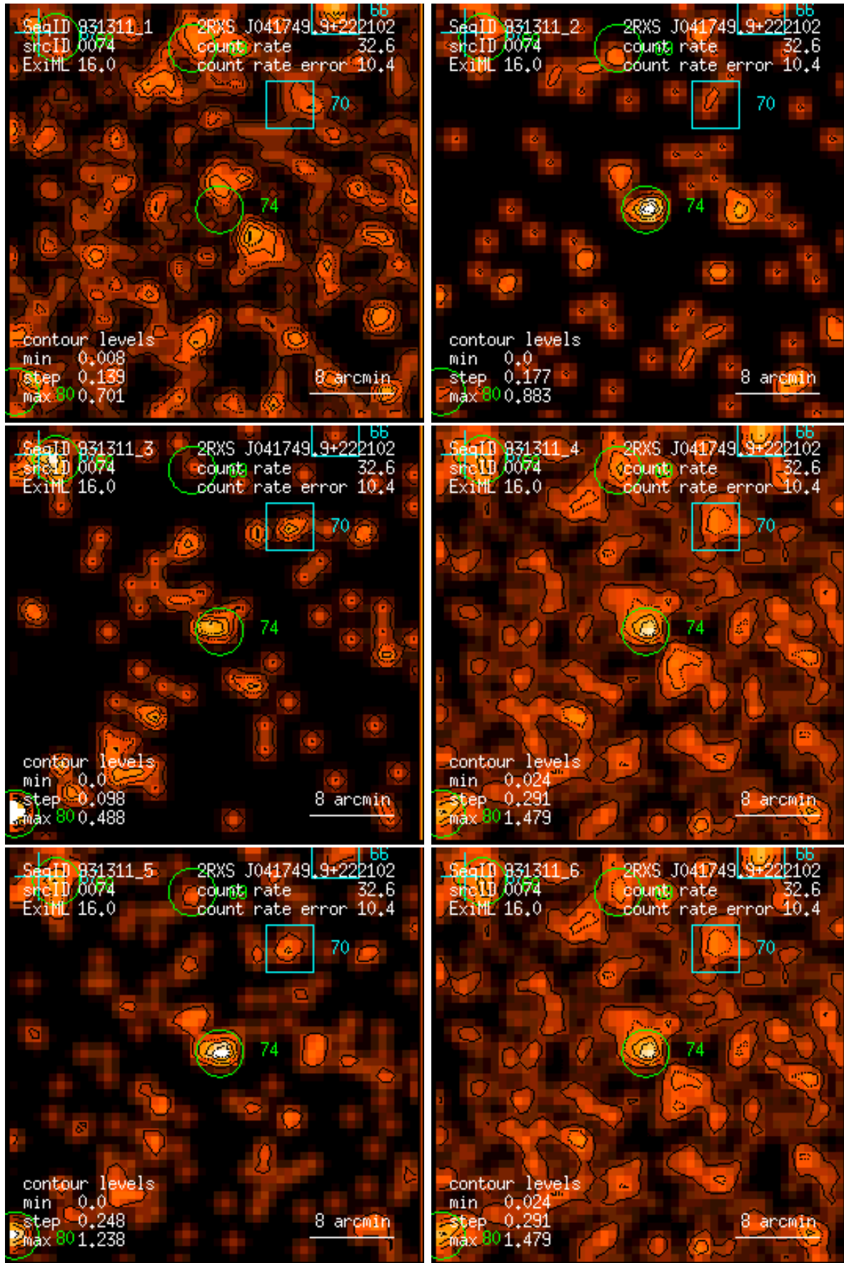
Figure 74: RASS 931311: detection 0074: band rate images, Gaussian filter: (1) PSPC channels 11 – 41, (2) 52 – 90, (3) 91 – 201, (4) 11 – 235, (5) 52 – 201, (6) 11 – 201. Broad band rates in counts/ks. Band rate contour levels in counts/ks/arcmin 2 .
