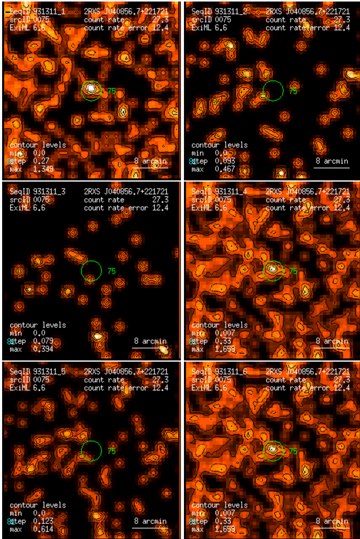
Figure 75: RASS 931311: detection 0075: band rate images, Gaussian filter: (1) PSPC channels 11 – 41, (2) 52 – 90, (3) 91 – 201, (4) 11 – 235, (5) 52 – 201, (6) 11 – 201. Broad band rates in counts/ks. Band rate contour levels in counts/ks/arcmin 2 .
