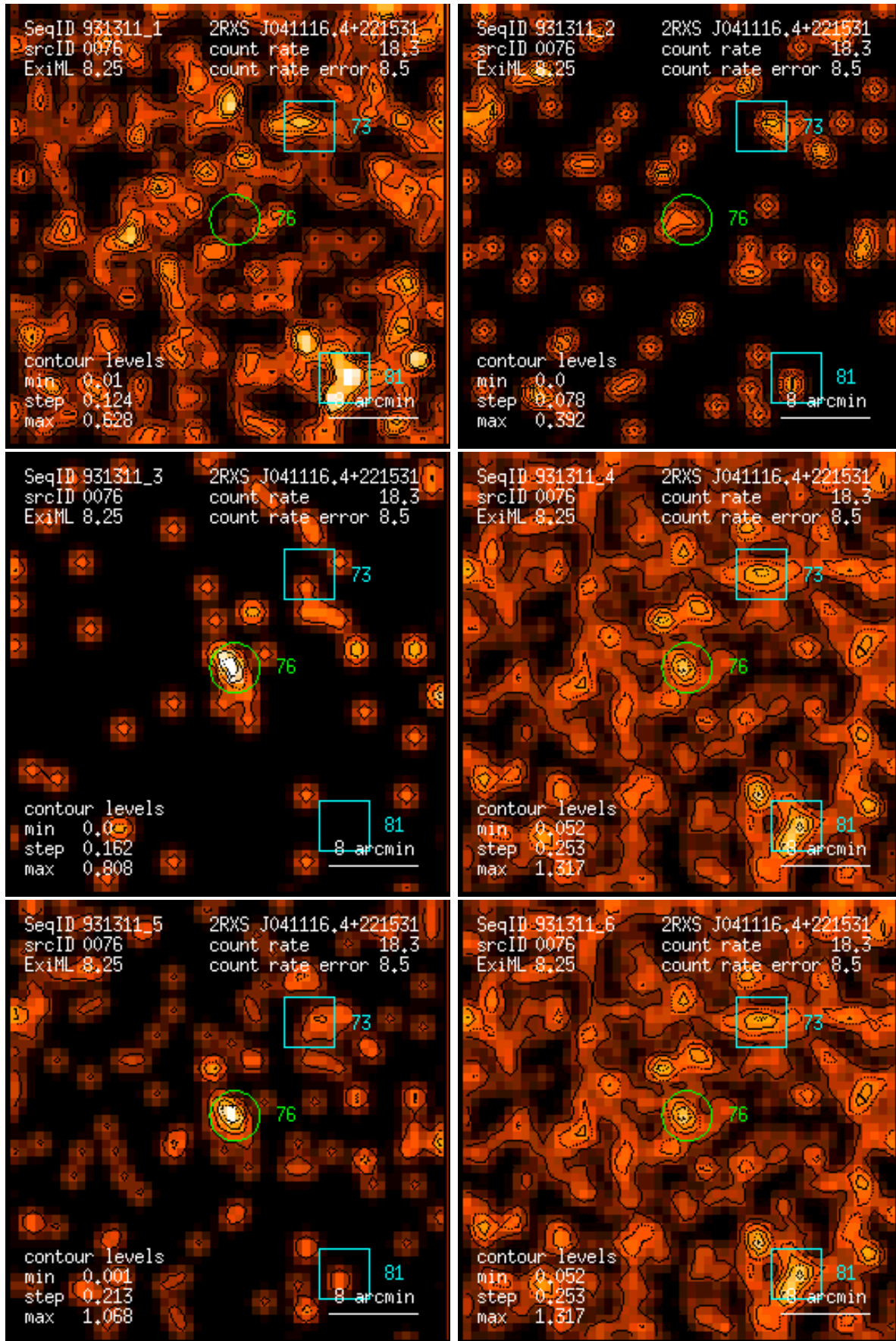
Figure 76: RASS 931311: detection 0076: band rate images, Gaussian filter: (1) PSPC channels 11 – 41, (2) 52 – 90, (3) 91 – 201, (4) 11 – 235, (5) 52 – 201, (6) 11 – 201. Broad band rates in counts/ks. Band rate contour levels in counts/ks/arcmin 2 .
