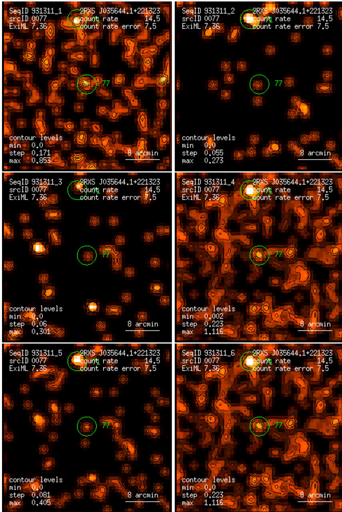
Figure 77: RASS 931311: detection 0077: band rate images, Gaussian filter: (1) PSPC channels 11 – 41, (2) 52 – 90, (3) 91 – 201, (4) 11 – 235, (5) 52 – 201, (6) 11 – 201. Broad band rates in counts/ks. Band rate contour levels in counts/ks/arcmin 2 .
