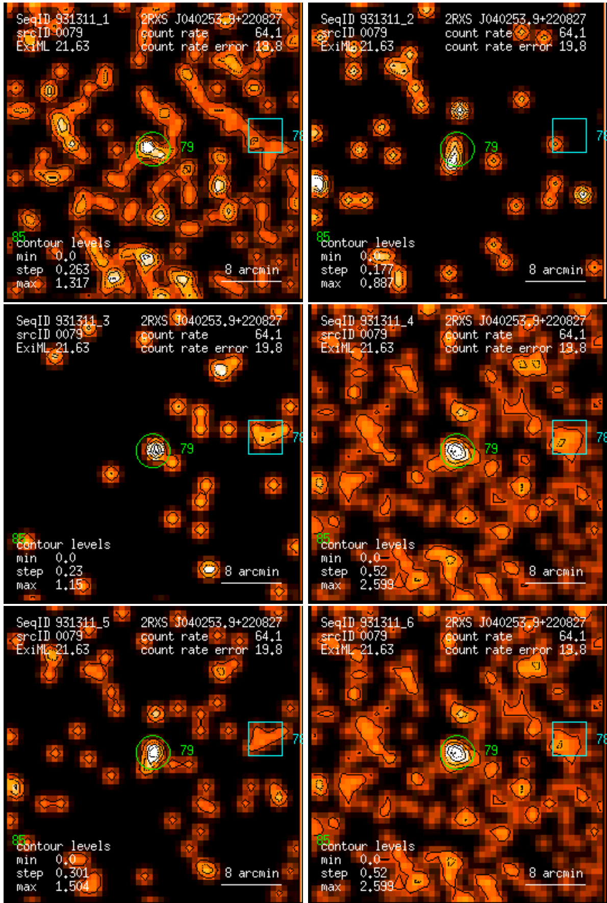
Figure 79: RASS 931311: detection 0079: band rate images, Gaussian filter: (1) PSPC channels 11 – 41, (2) 52 – 90, (3) 91 – 201, (4) 11 – 235, (5) 52 – 201, (6) 11 – 201. Broad band rates in counts/ks. Band rate contour levels in counts/ks/arcmin 2 .
