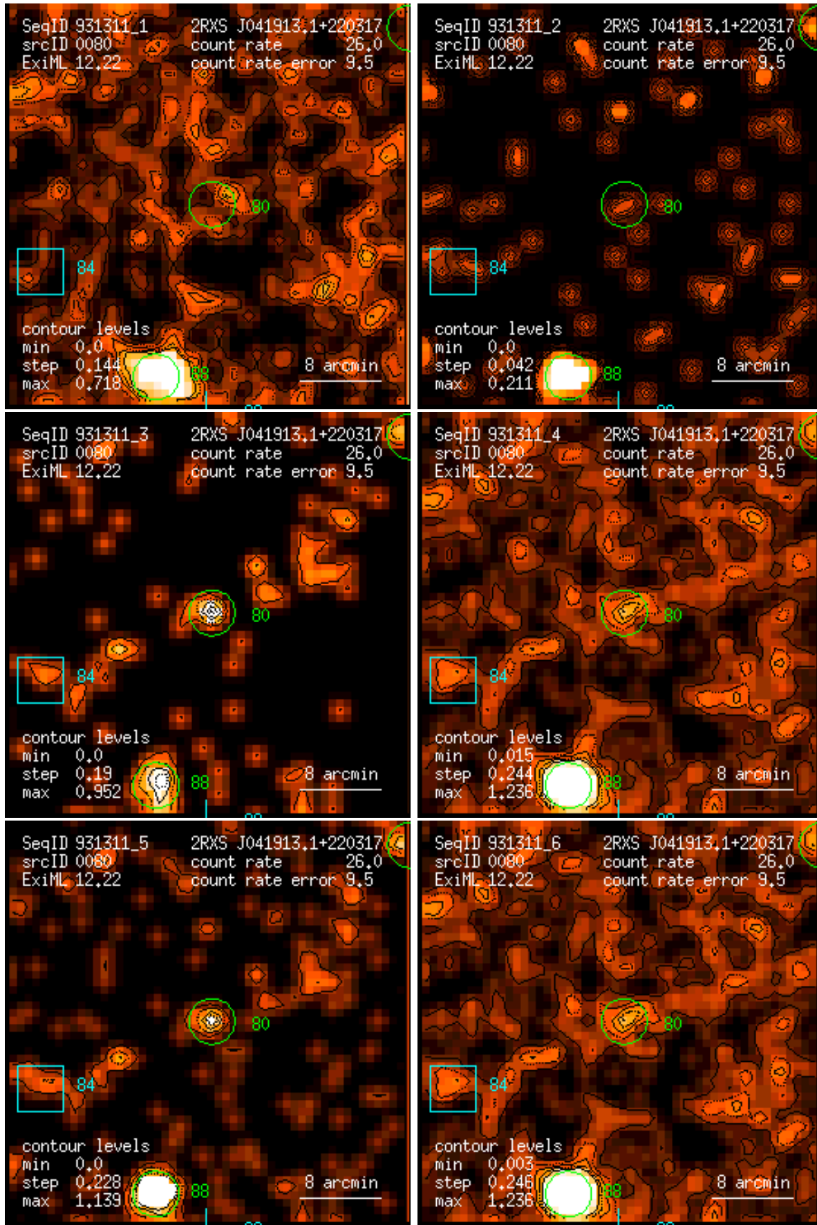
Figure 80: RASS 931311: detection 0080: band rate images, Gaussian filter: (1) PSPC channels 11 – 41, (2) 52 – 90, (3) 91 – 201, (4) 11 – 235, (5) 52 – 201, (6) 11 – 201. Broad band rates in counts/ks. Band rate contour levels in counts/ks/arcmin 2 .
