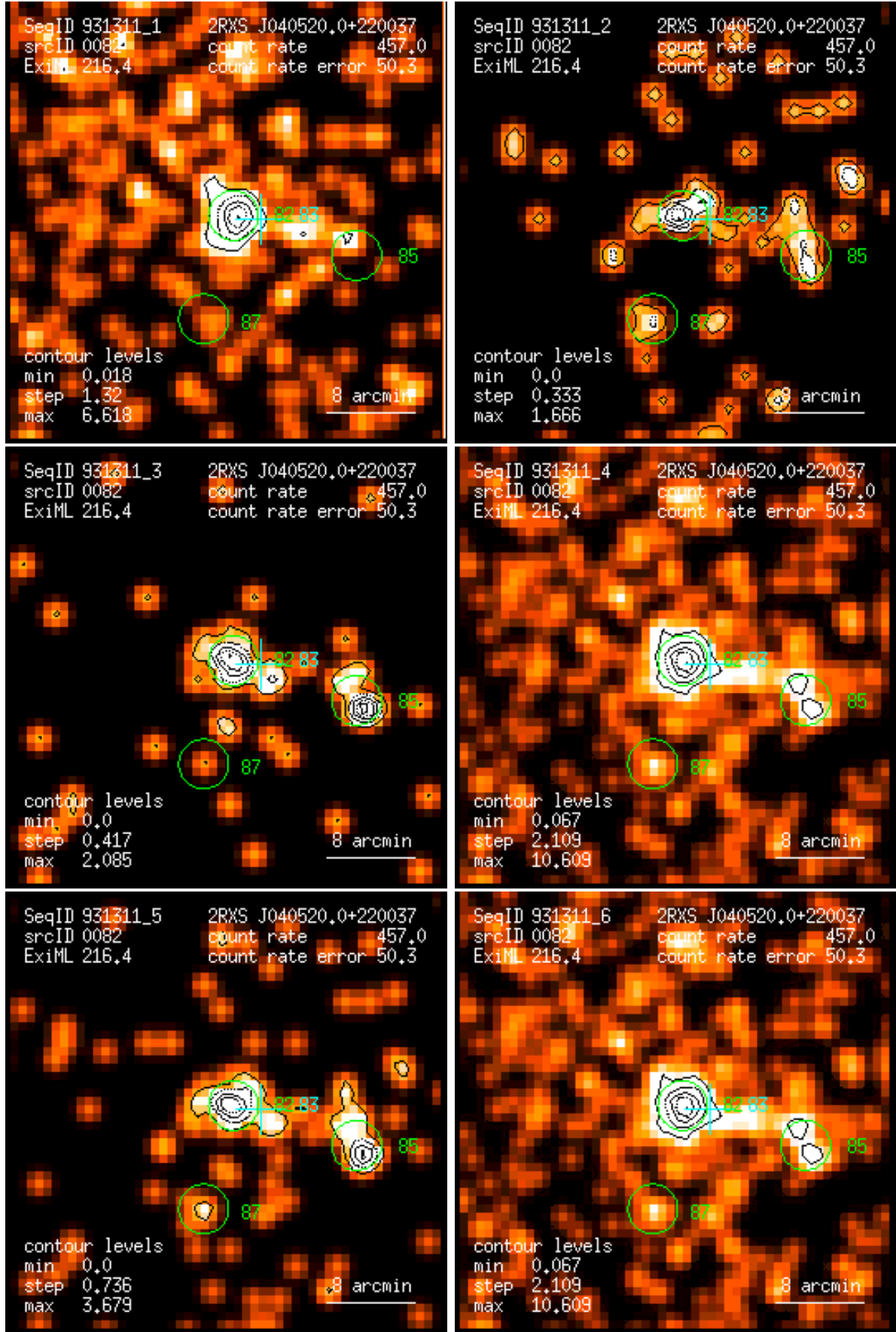
Figure 82: RASS 931311: detection 0082: band rate images, Gaussian filter: (1) PSPC channels 11 – 41, (2) 52 – 90, (3) 91 – 201, (4) 11 – 235, (5) 52 – 201, (6) 11 – 201. Broad band rates in counts/ks. Band rate contour levels in counts/ks/arcmin 2 .
