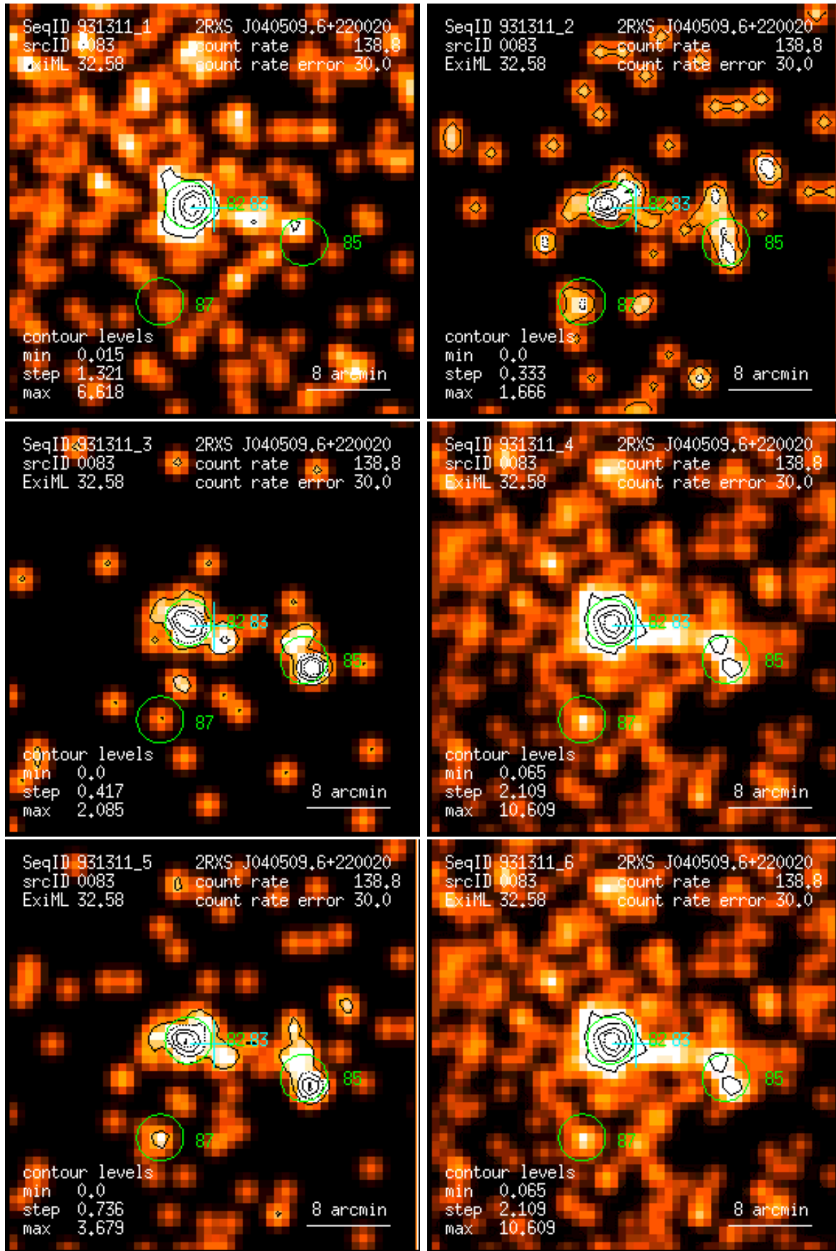
Figure 83: RASS 931311: detection 0083: band rate images, Gaussian filter: (1) PSPC channels 11 – 41, (2) 52 – 90, (3) 91 – 201, (4) 11 – 235, (5) 52 – 201, (6) 11 – 201. Broad band rates in counts/ks. Band rate contour levels in counts/ks/arcmin 2 .
