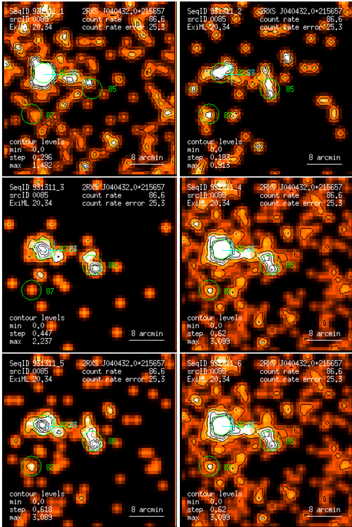
Figure 85: RASS 931311: detection 0085: band rate images, Gaussian filter: (1) PSPC channels 11 – 41, (2) 52 – 90, (3) 91 – 201, (4) 11 – 235, (5) 52 – 201, (6) 11 – 201. Broad band rates in counts/ks. Band rate contour levels in counts/ks/arcmin 2 .
