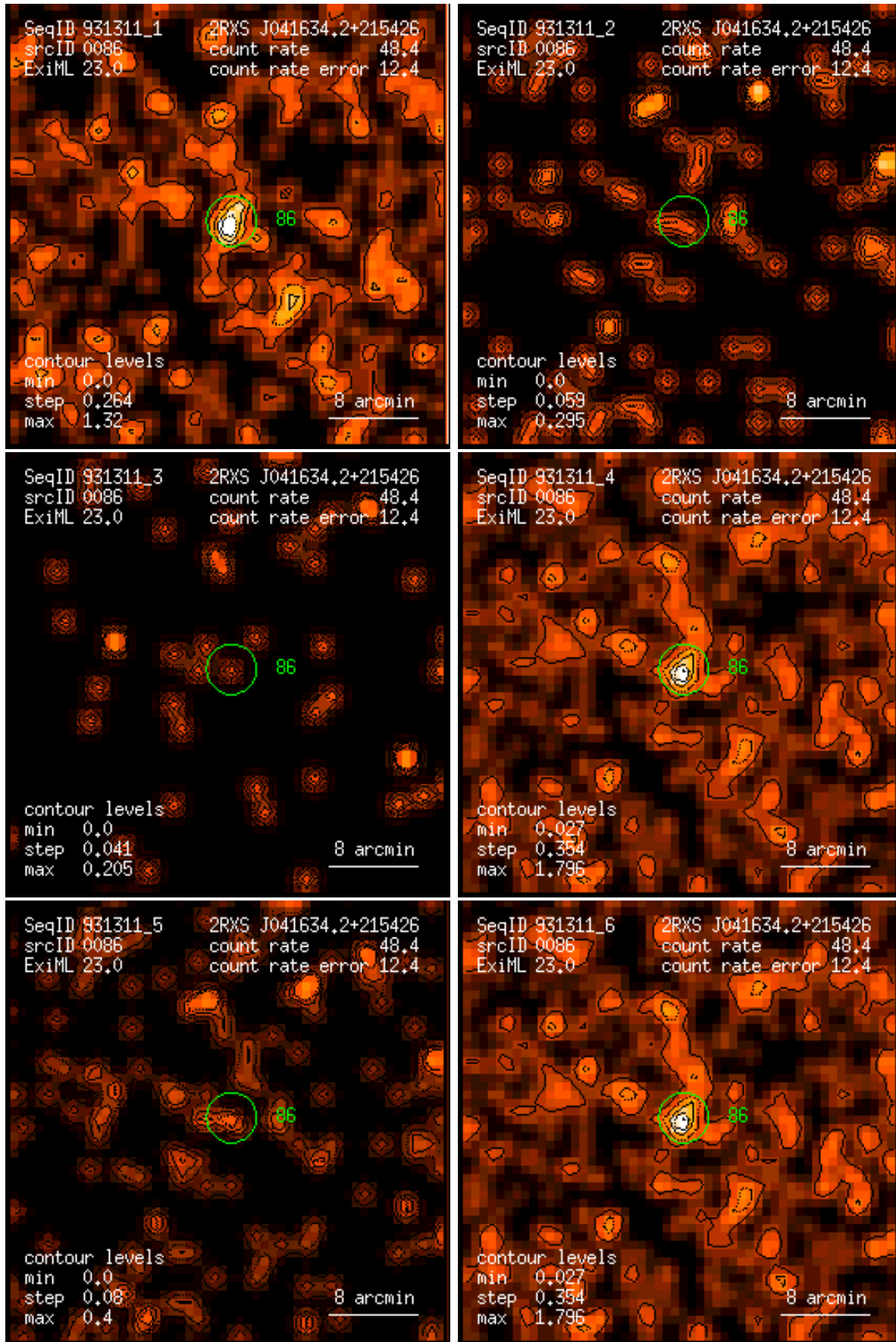
Figure 86: RASS 931311: detection 0086: band rate images, Gaussian filter: (1) PSPC channels 11 – 41, (2) 52 – 90, (3) 91 – 201, (4) 11 – 235, (5) 52 – 201, (6) 11 – 201. Broad band rates in counts/ks. Band rate contour levels in counts/ks/arcmin 2 .
