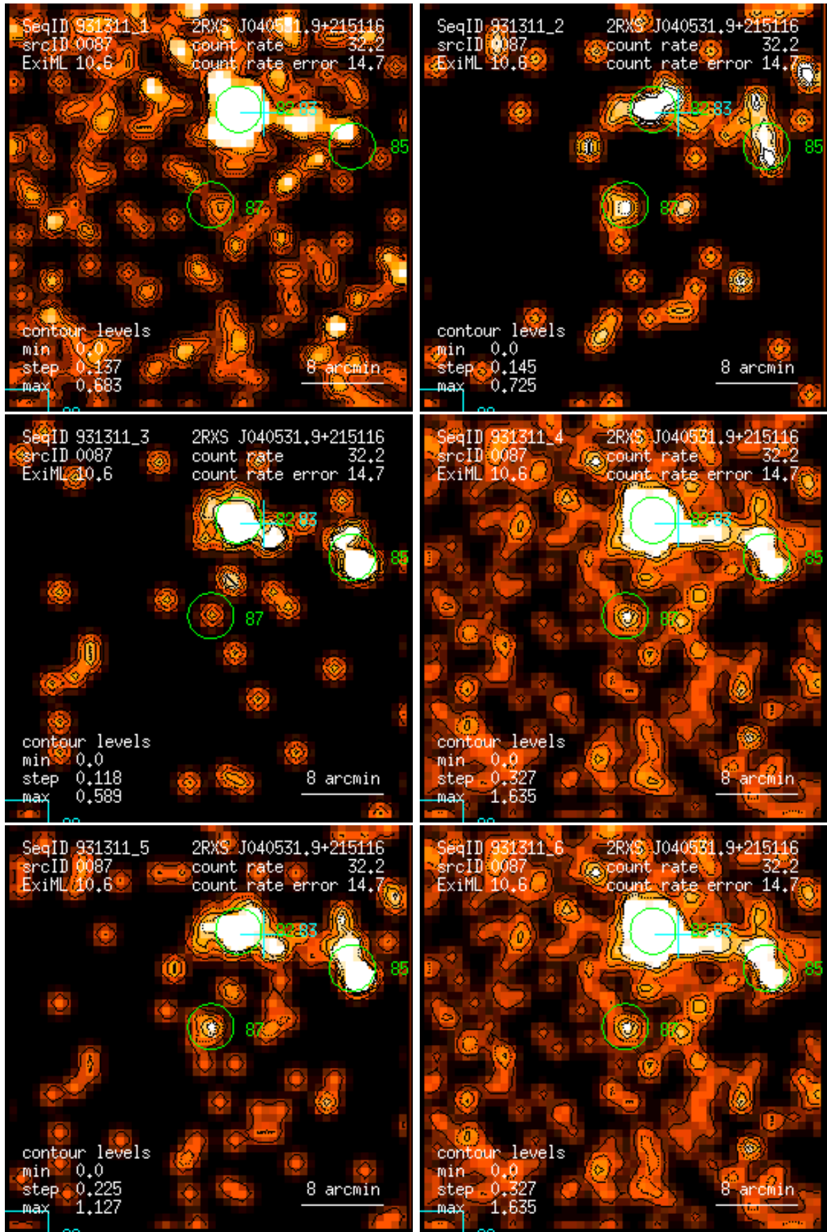
Figure 87: RASS 931311: detection 0087: band rate images, Gaussian filter: (1) PSPC channels 11 – 41, (2) 52 – 90, (3) 91 – 201, (4) 11 – 235, (5) 52 – 201, (6) 11 – 201. Broad band rates in counts/ks. Band rate contour levels in counts/ks/arcmin 2 .
