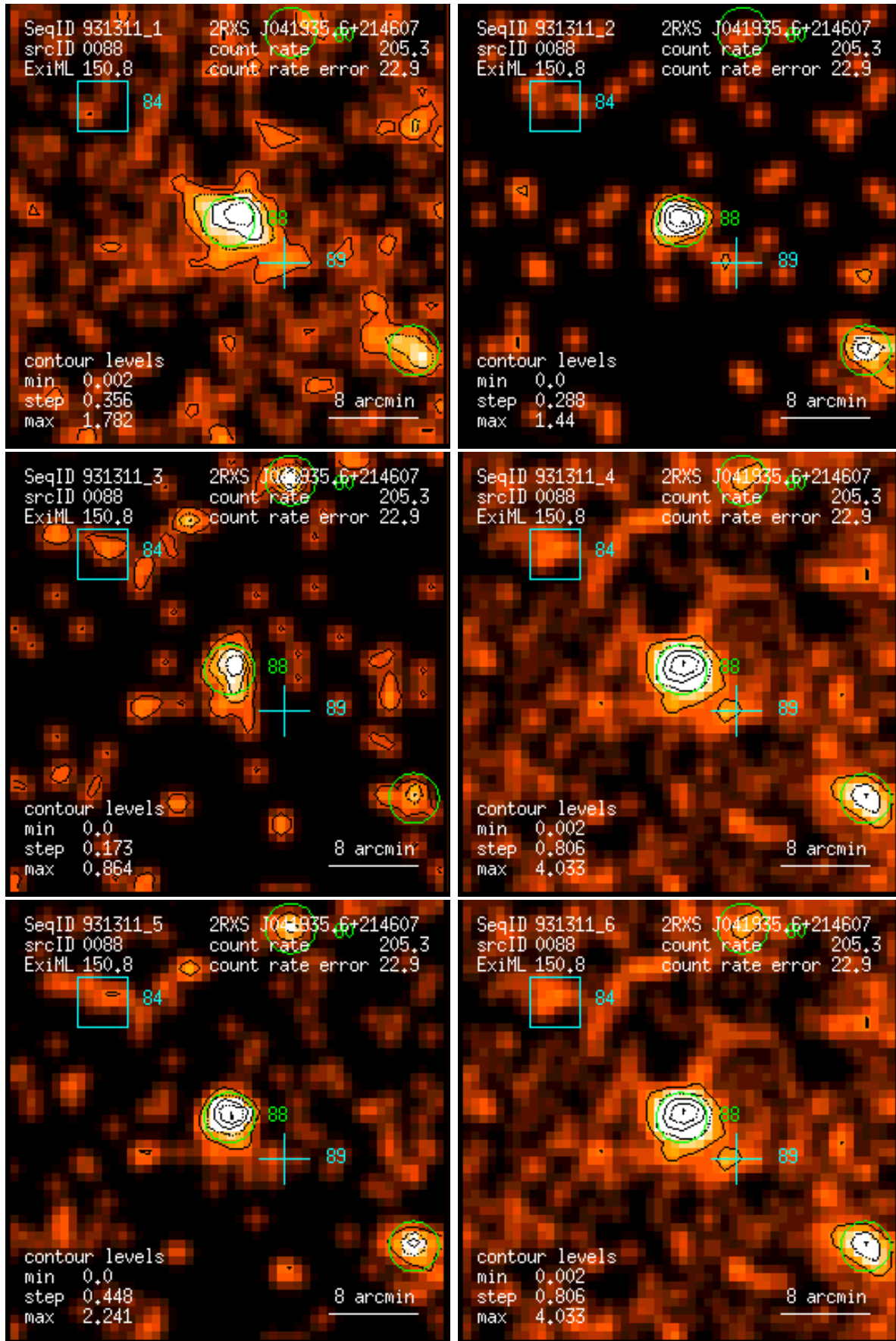
Figure 88: RASS 931311: detection 0088: band rate images, Gaussian filter: (1) PSPC channels 11 – 41, (2) 52 – 90, (3) 91 – 201, (4) 11 – 235, (5) 52 – 201, (6) 11 – 201. Broad band rates in counts/ks. Band rate contour levels in counts/ks/arcmin 2 .
