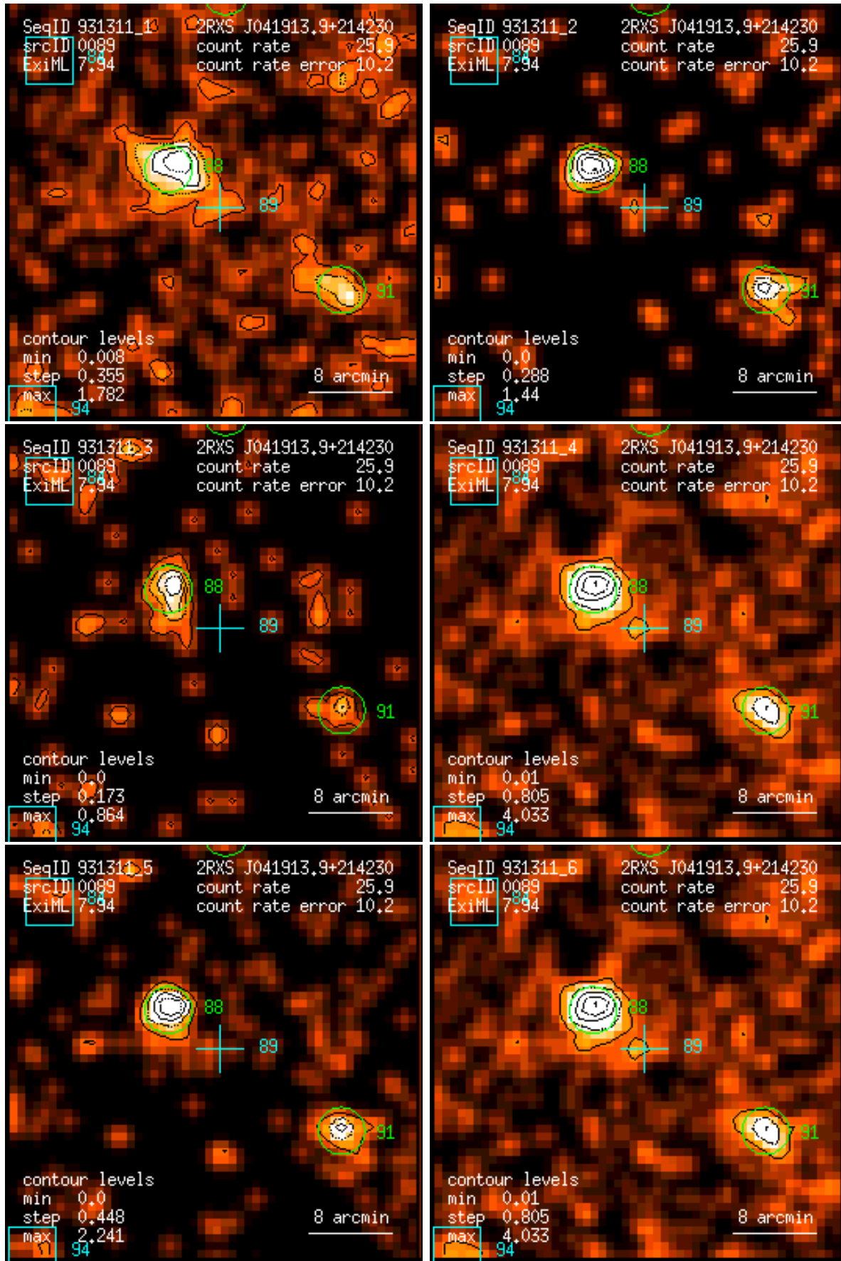
Figure 89: RASS 931311: detection 0089: band rate images, Gaussian filter: (1) PSPC channels 11 – 41, (2) 52 – 90, (3) 91 – 201, (4) 11 – 235, (5) 52 – 201, (6) 11 – 201. Broad band rates in counts/ks. Band rate contour levels in counts/ks/arcmin 2 .
