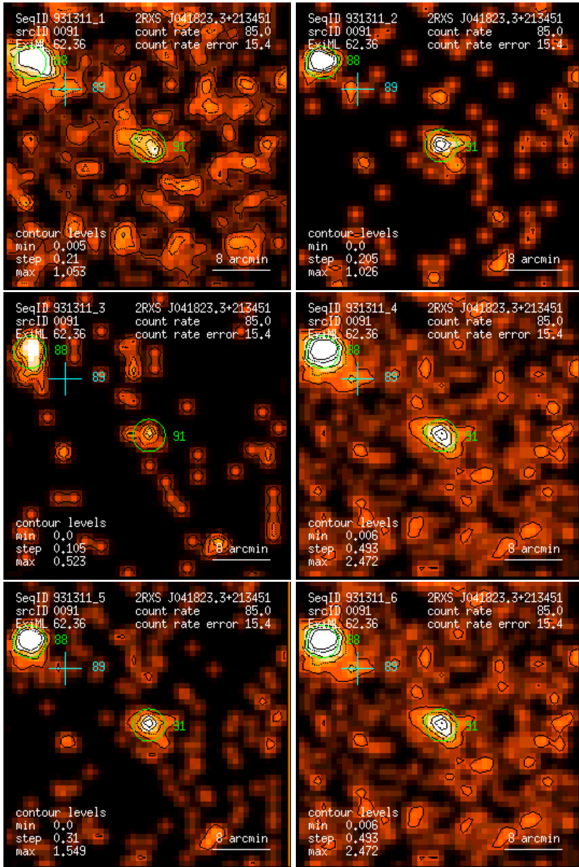
Figure 91: RASS 931311: detection 0091: band rate images, Gaussian filter: (1) PSPC channels 11 – 41, (2) 52 – 90, (3) 91 – 201, (4) 11 – 235, (5) 52 – 201, (6) 11 – 201. Broad band rates in counts/ks. Band rate contour levels in counts/ks/arcmin 2 .
