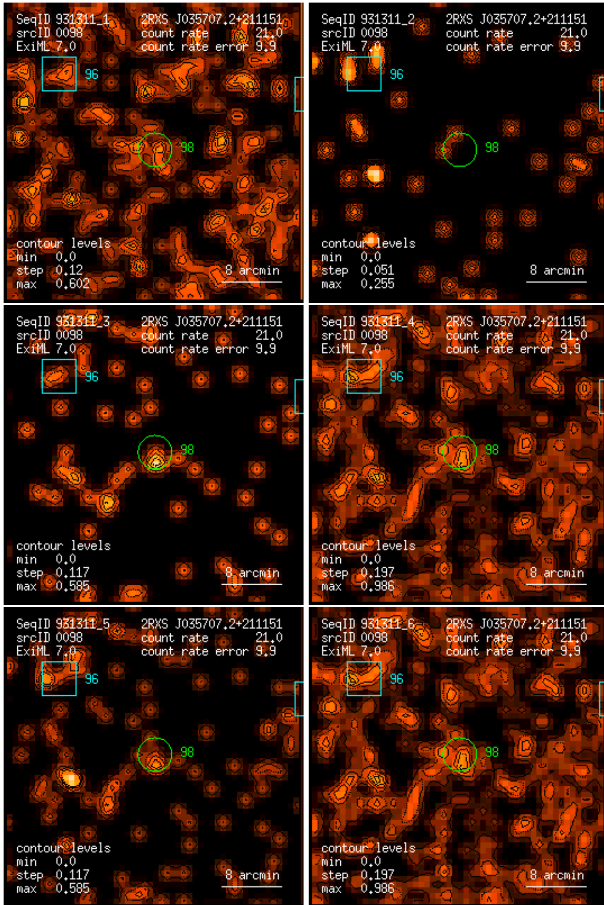
Figure 98: RASS 931311: detection 0098: band rate images, Gaussian filter: (1) PSPC channels 11 – 41, (2) 52 – 90, (3) 91 – 201, (4) 11 – 235, (5) 52 – 201, (6) 11 – 201. Broad band rates in counts/ks. Band rate contour levels in counts/ks/arcmin 2 .
