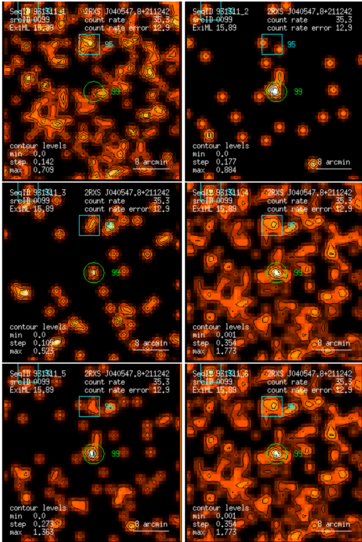
Figure 99: RASS 931311: detection 0099: band rate images, Gaussian filter: (1) PSPC channels 11 – 41, (2) 52 – 90, (3) 91 – 201, (4) 11 – 235, (5) 52 – 201, (6) 11 – 201. Broad band rates in counts/ks. Band rate contour levels in counts/ks/arcmin 2 .
