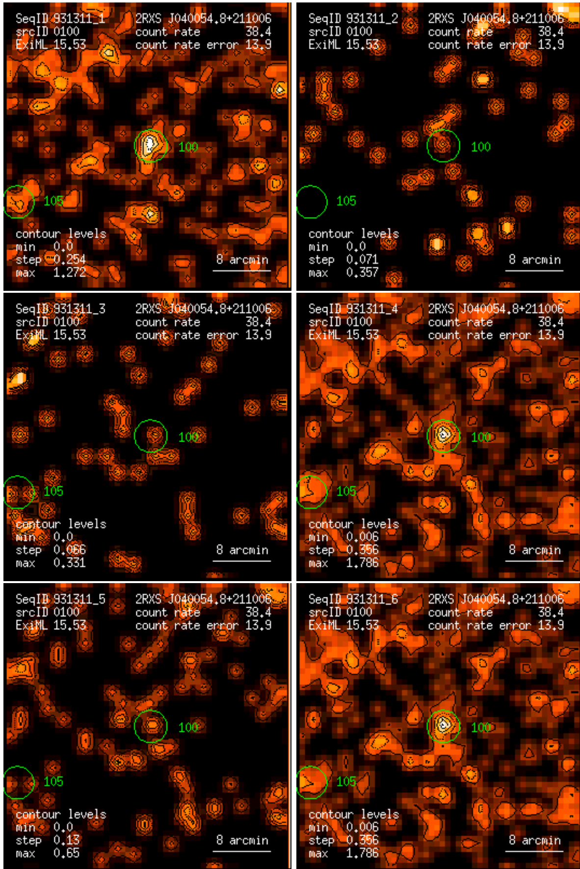
Figure 100: RASS 931311: detection 0100: band rate images, Gaussian filter: (1) PSPC channels 11 – 41, (2) 52 – 90, (3) 91 – 201, (4) 11 – 235, (5) 52 – 201, (6) 11 – 201. Broad band rates in counts/ks. Band rate contour levels in counts/ks/arcmin 2 .
