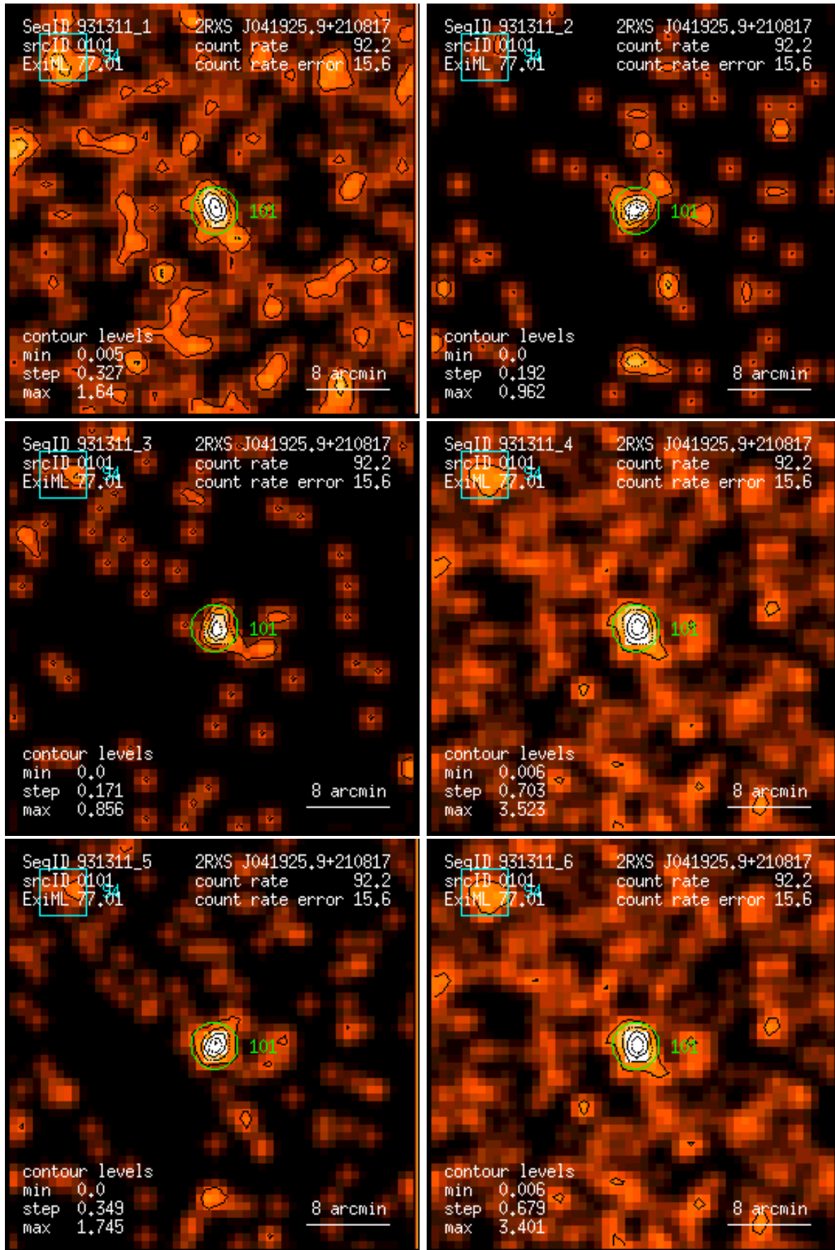
Figure 101: RASS 931311: detection 0101: band rate images, Gaussian filter: (1) PSPC channels 11 – 41, (2) 52 – 90, (3) 91 – 201, (4) 11 – 235, (5) 52 – 201, (6) 11 – 201. Broad band rates in counts/ks. Band rate contour levels in counts/ks/arcmin 2 .
