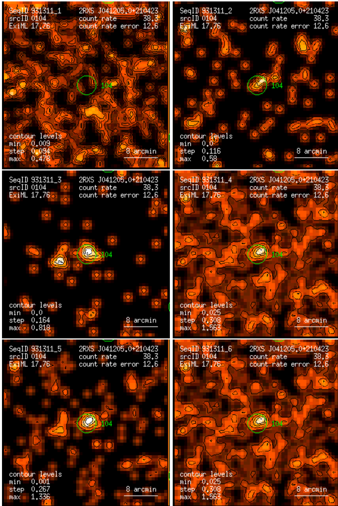
Figure 104: RASS 931311: detection 0104: band rate images, Gaussian filter: (1) PSPC channels 11 – 41, (2) 52 – 90, (3) 91 – 201, (4) 11 – 235, (5) 52 – 201, (6) 11 – 201. Broad band rates in counts/ks. Band rate contour levels in counts/ks/arcmin 2 .
