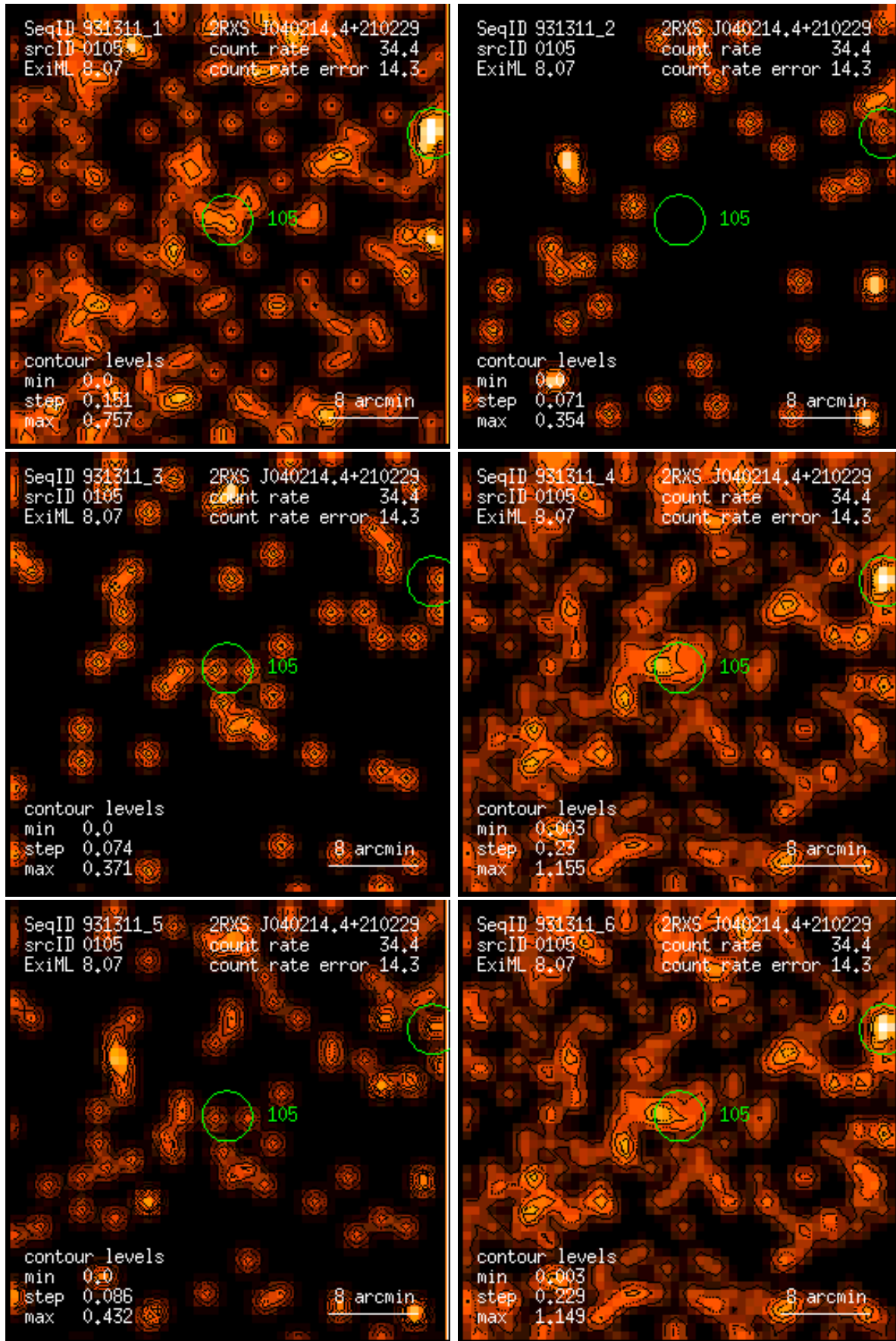
Figure 105: RASS 931311: detection 0105: band rate images, Gaussian filter: (1) PSPC channels 11 – 41, (2) 52 – 90, (3) 91 – 201, (4) 11 – 235, (5) 52 – 201, (6) 11 – 201. Broad band rates in counts/ks. Band rate contour levels in counts/ks/arcmin 2 .
