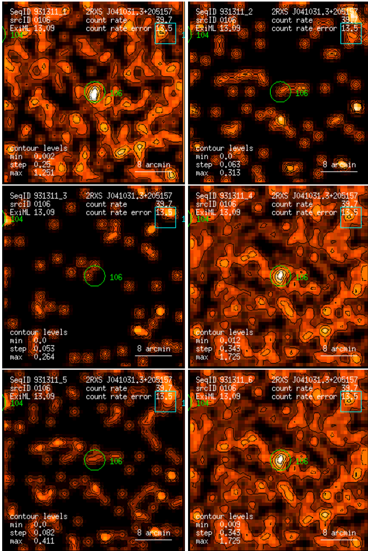
Figure 106: RASS 931311: detection 0106: band rate images, Gaussian filter: (1) PSPC channels 11 – 41, (2) 52 – 90, (3) 91 – 201, (4) 11 – 235, (5) 52 – 201, (6) 11 – 201. Broad band rates in counts/ks. Band rate contour levels in counts/ks/arcmin 2 .
