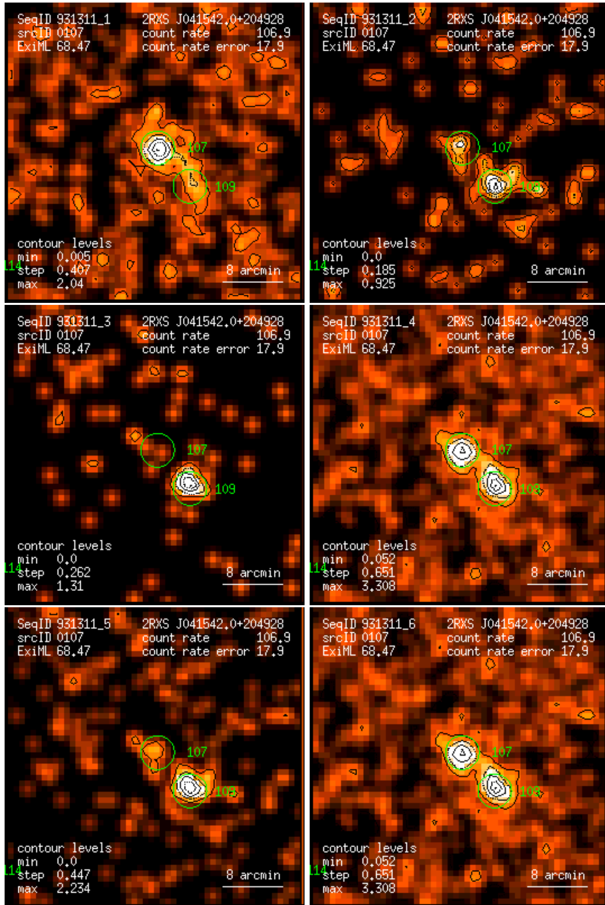
Figure 107: RASS 931311: detection 0107: band rate images, Gaussian filter: (1) PSPC channels 11 – 41, (2) 52 – 90, (3) 91 – 201, (4) 11 – 235, (5) 52 – 201, (6) 11 – 201. Broad band rates in counts/ks. Band rate contour levels in counts/ks/arcmin 2 .
