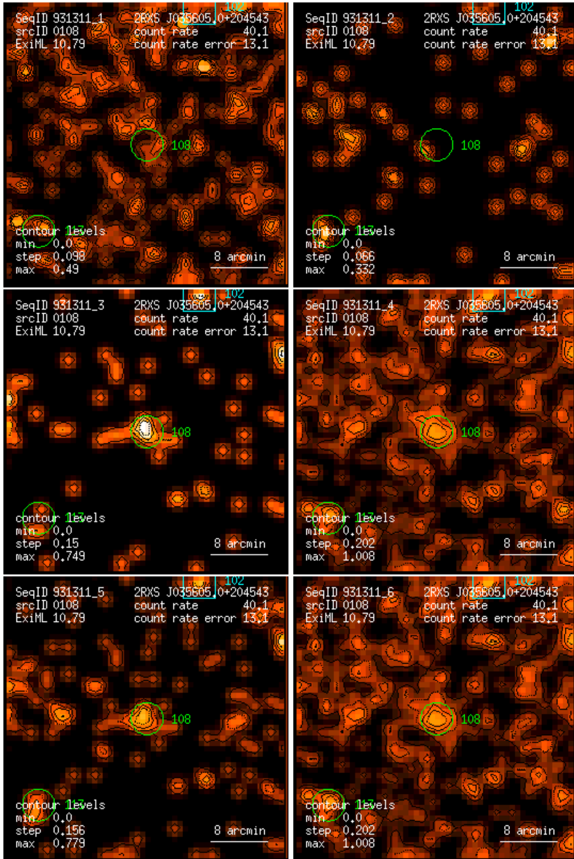
Figure 108: RASS 931311: detection 0108: band rate images, Gaussian filter: (1) PSPC channels 11 – 41, (2) 52 – 90, (3) 91 – 201, (4) 11 – 235, (5) 52 – 201, (6) 11 – 201. Broad band rates in counts/ks. Band rate contour levels in counts/ks/arcmin 2 .
