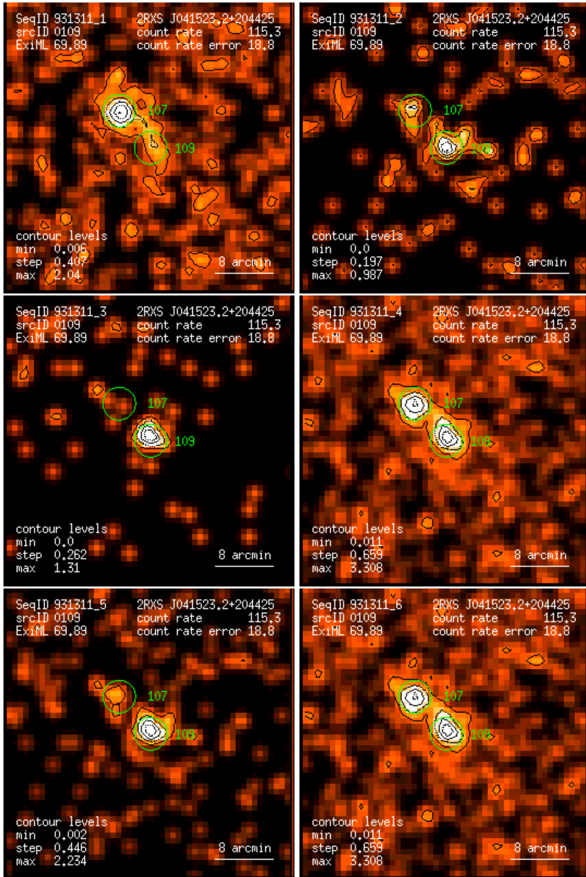
Figure 109: RASS 931311: detection 0109: band rate images, Gaussian filter: (1) PSPC channels 11 – 41, (2) 52 – 90, (3) 91 – 201, (4) 11 – 235, (5) 52 – 201, (6) 11 – 201. Broad band rates in counts/ks. Band rate contour levels in counts/ks/arcmin 2 .
