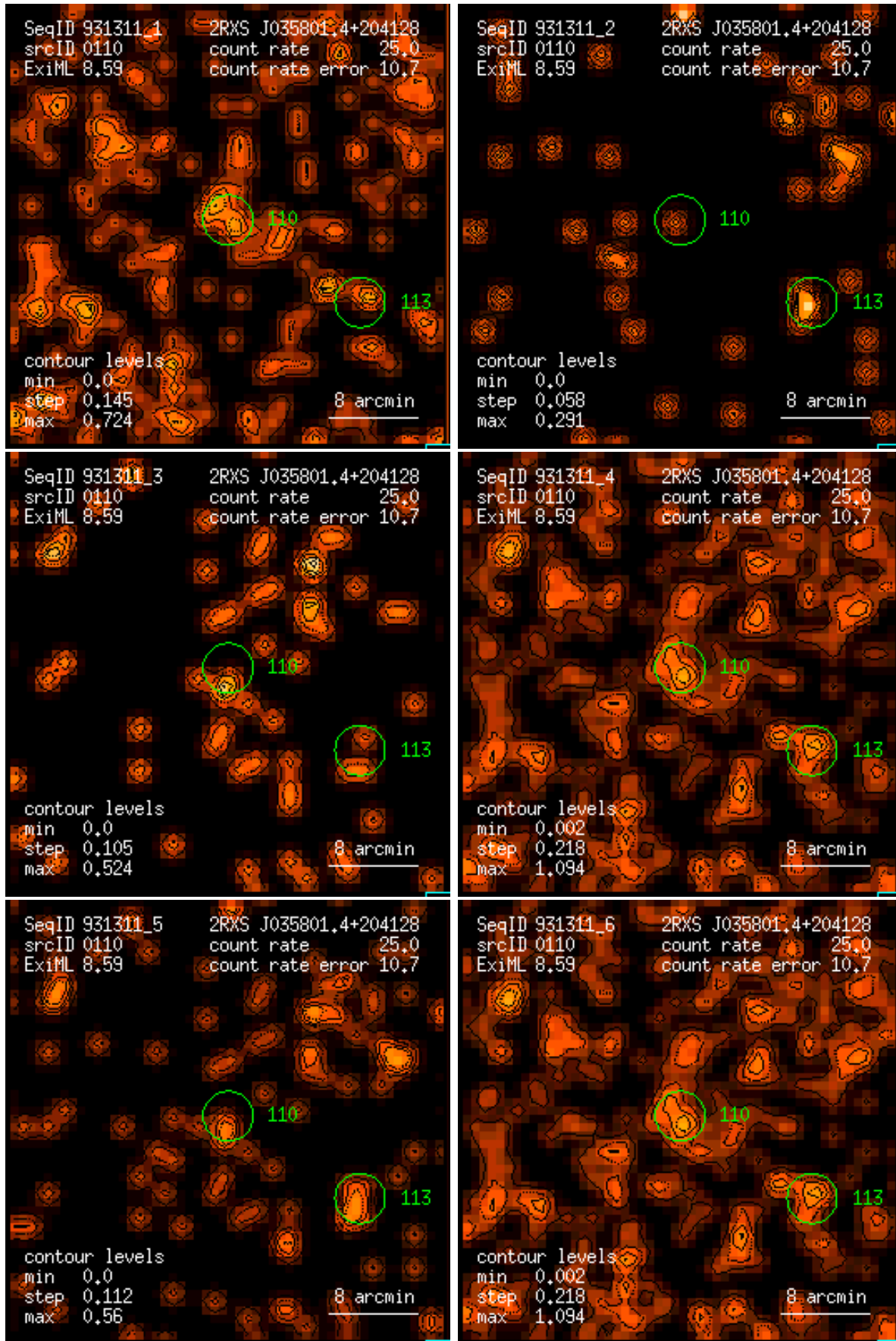
Figure 110: RASS 931311: detection 0110: band rate images, Gaussian filter: (1) PSPC channels 11 – 41, (2) 52 – 90, (3) 91 – 201, (4) 11 – 235, (5) 52 – 201, (6) 11 – 201. Broad band rates in counts/ks. Band rate contour levels in counts/ks/arcmin 2 .
