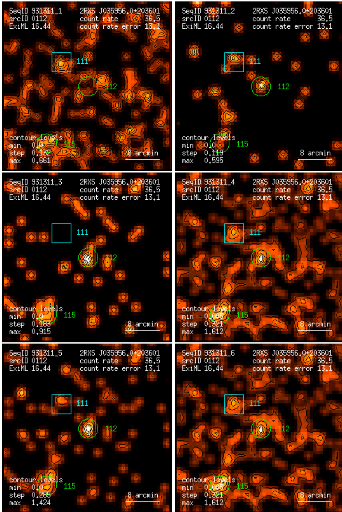
Figure 112: RASS 931311: detection 0112: band rate images, Gaussian filter: (1) PSPC channels 11 – 41, (2) 52 – 90, (3) 91 – 201, (4) 11 – 235, (5) 52 – 201, (6) 11 – 201. Broad band rates in counts/ks. Band rate contour levels in counts/ks/arcmin 2 .
