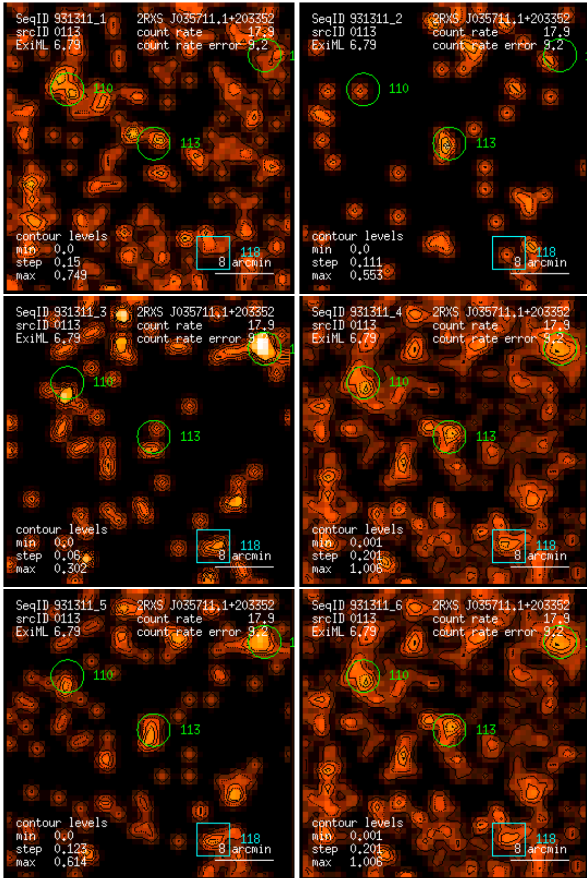
Figure 113: RASS 931311: detection 0113: band rate images, Gaussian filter: (1) PSPC channels 11 – 41, (2) 52 – 90, (3) 91 – 201, (4) 11 – 235, (5) 52 – 201, (6) 11 – 201. Broad band rates in counts/ks. Band rate contour levels in counts/ks/arcmin 2 .
