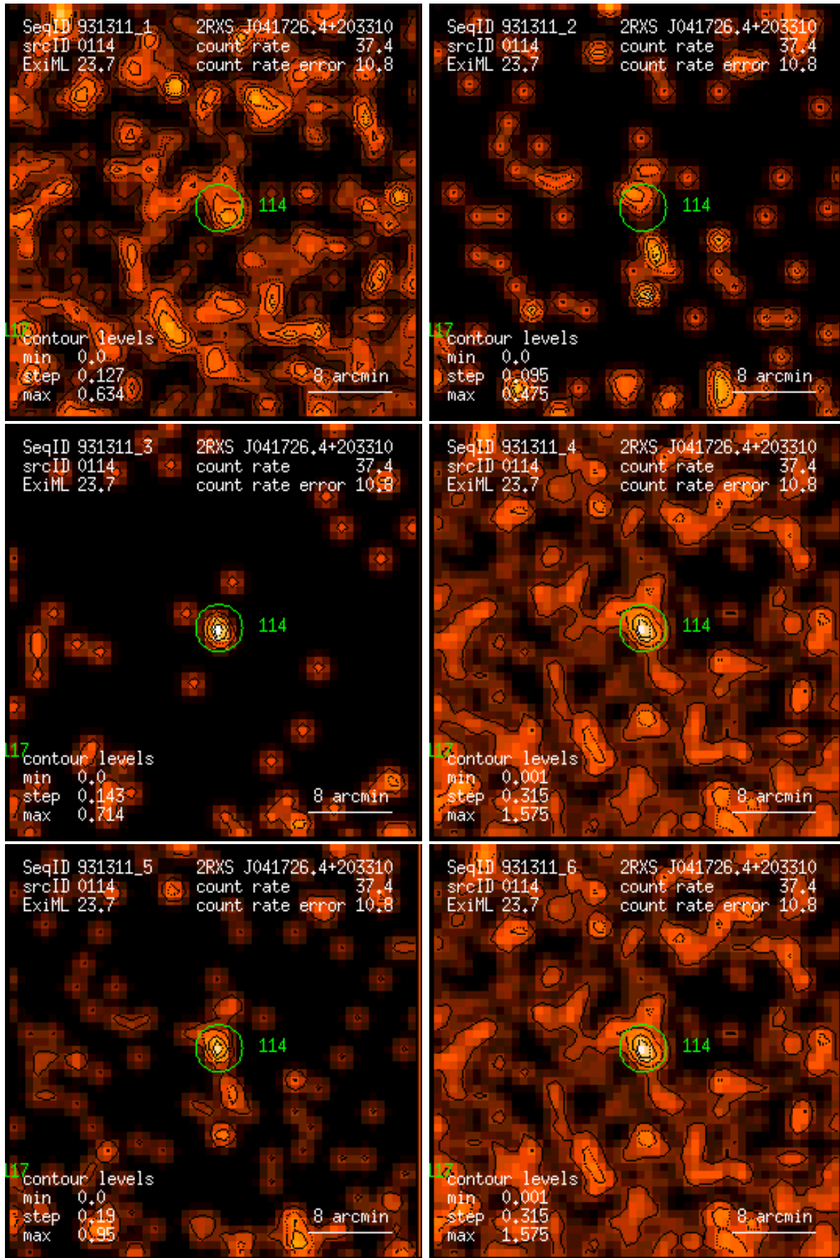
Figure 114: RASS 931311: detection 0114: band rate images, Gaussian filter: (1) PSPC channels 11 – 41, (2) 52 – 90, (3) 91 – 201, (4) 11 – 235, (5) 52 – 201, (6) 11 – 201. Broad band rates in counts/ks. Band rate contour levels in counts/ks/arcmin 2 .
