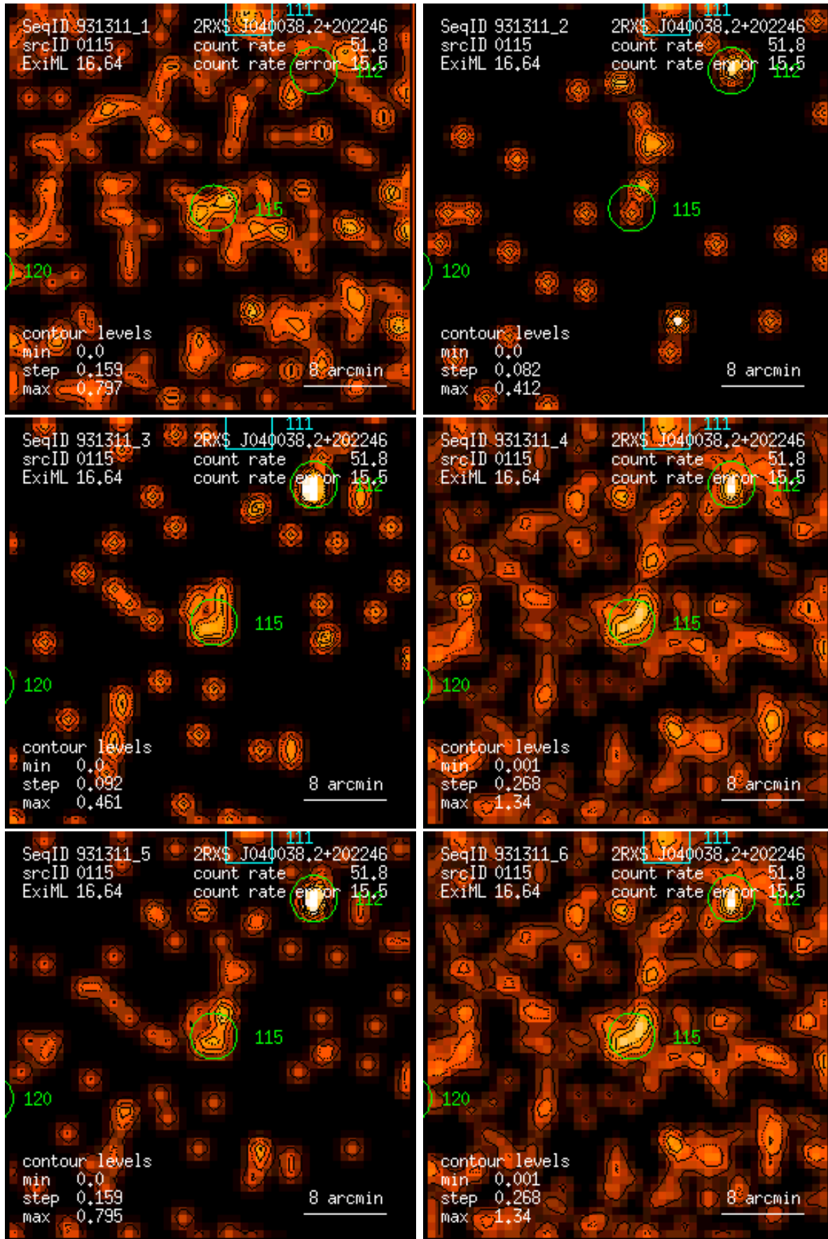
Figure 115: RASS 931311: detection 0115: band rate images, Gaussian filter: (1) PSPC channels 11 – 41, (2) 52 – 90, (3) 91 – 201, (4) 11 – 235, (5) 52 – 201, (6) 11 – 201. Broad band rates in counts/ks. Band rate contour levels in counts/ks/arcmin 2 .
