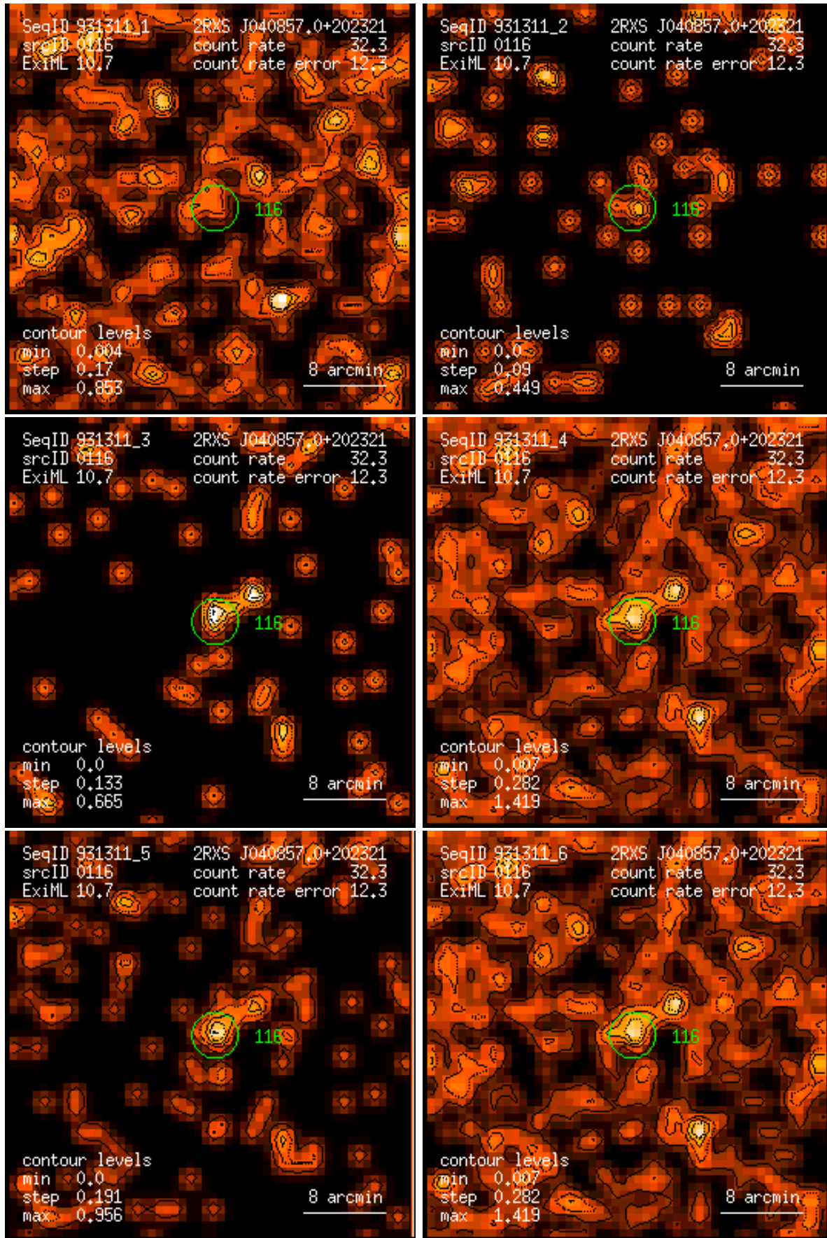
Figure 116: RASS 931311: detection 0116: band rate images, Gaussian filter: (1) PSPC channels 11 – 41, (2) 52 – 90, (3) 91 – 201, (4) 11 – 235, (5) 52 – 201, (6) 11 – 201. Broad band rates in counts/ks. Band rate contour levels in counts/ks/arcmin 2 .
