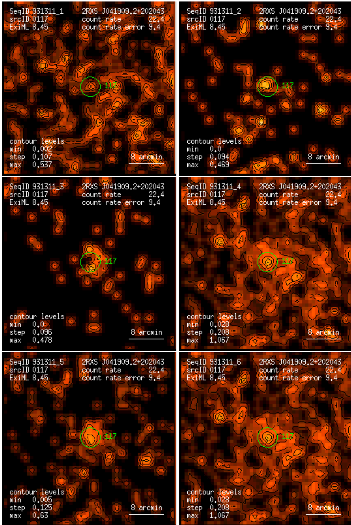
Figure 117: RASS 931311: detection 0117: band rate images, Gaussian filter: (1) PSPC channels 11 – 41, (2) 52 – 90, (3) 91 – 201, (4) 11 – 235, (5) 52 – 201, (6) 11 – 201. Broad band rates in counts/ks. Band rate contour levels in counts/ks/arcmin 2 .
