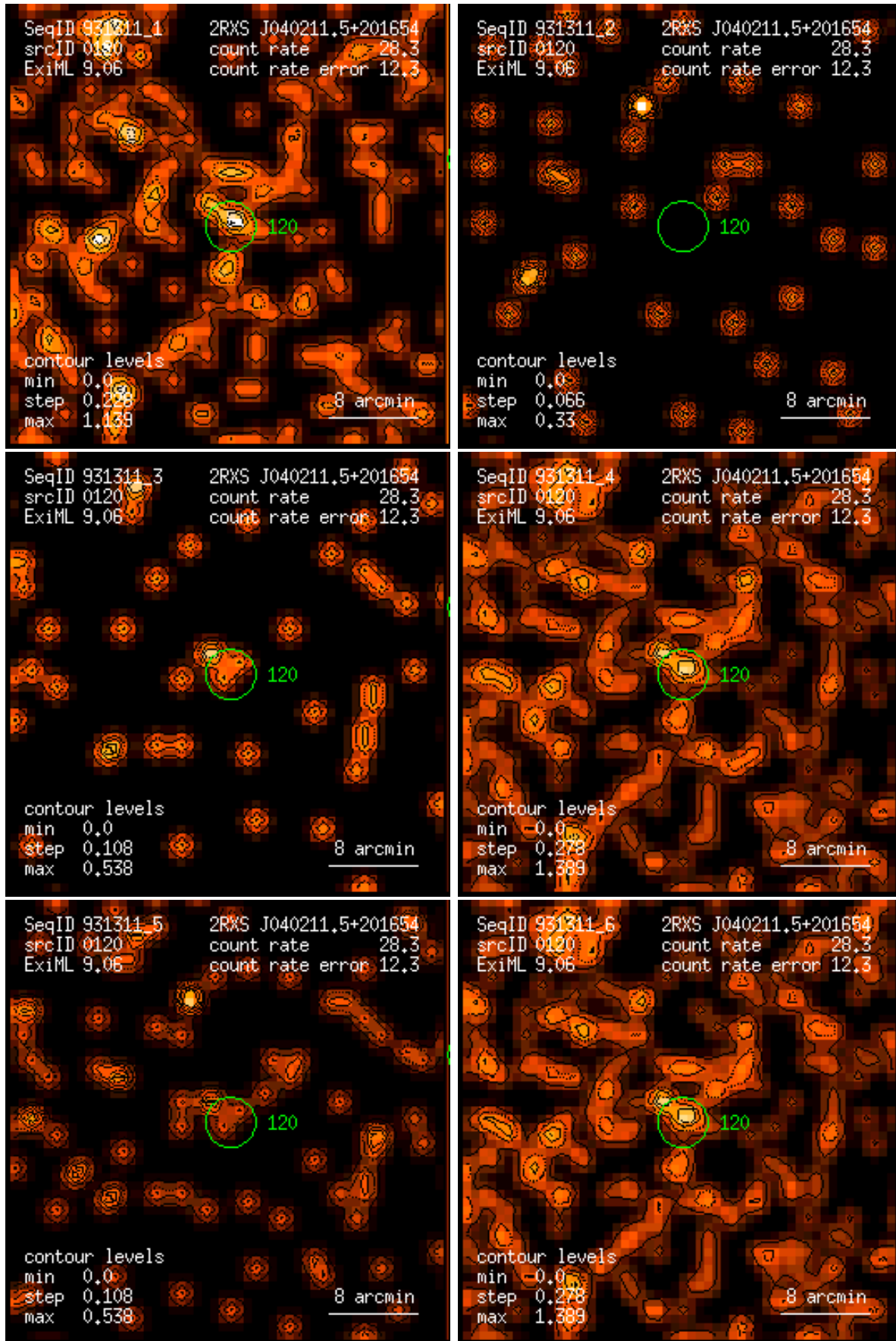
Figure 120: RASS 931311: detection 0120: band rate images, Gaussian filter: (1) PSPC channels 11 – 41, (2) 52 – 90, (3) 91 – 201, (4) 11 – 235, (5) 52 – 201, (6) 11 – 201. Broad band rates in counts/ks. Band rate contour levels in counts/ks/arcmin 2 .
