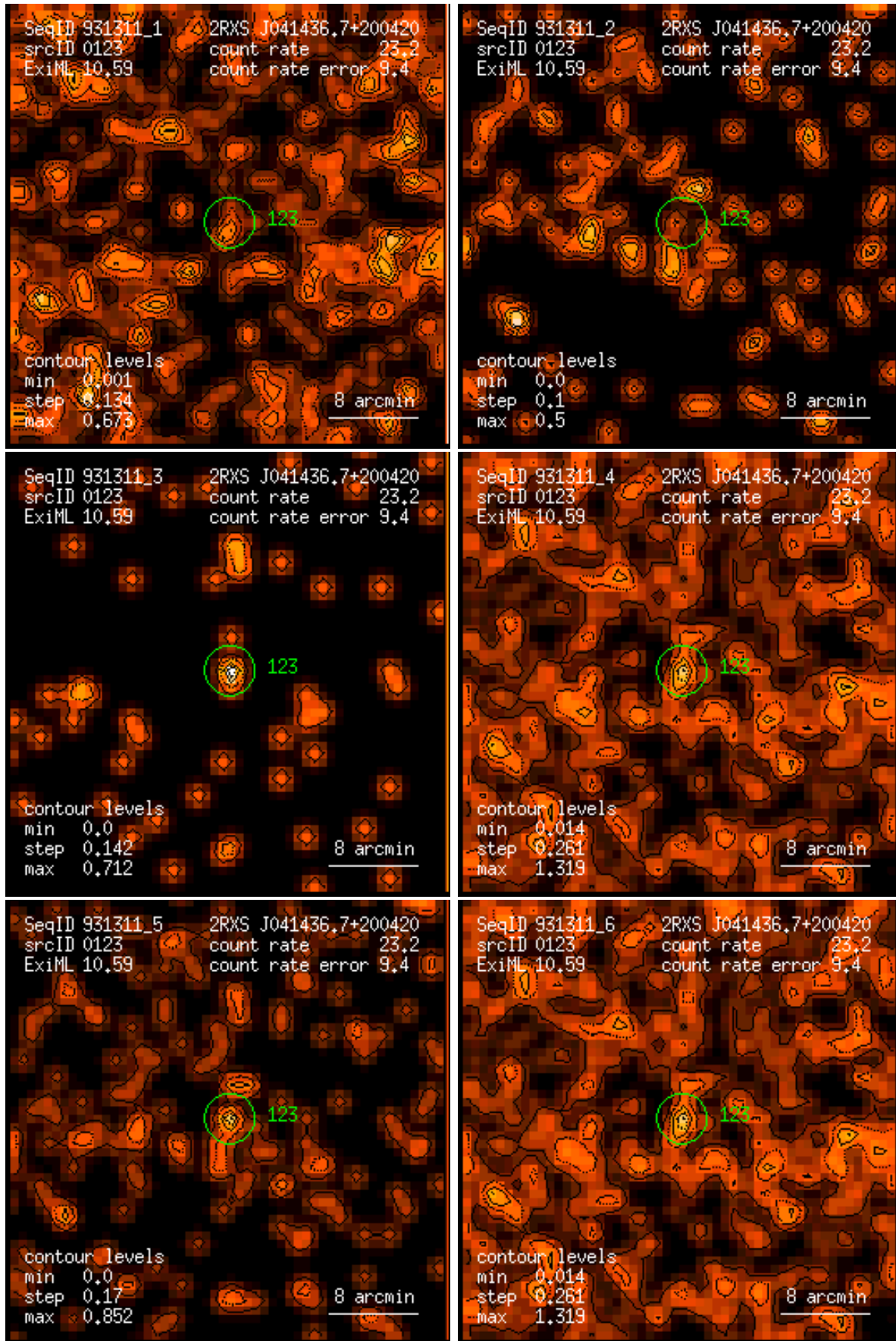
Figure 123: RASS 931311: detection 0123: band rate images, Gaussian filter: (1) PSPC channels 11 – 41, (2) 52 – 90, (3) 91 – 201, (4) 11 – 235, (5) 52 – 201, (6) 11 – 201. Broad band rates in counts/ks. Band rate contour levels in counts/ks/arcmin 2 .
